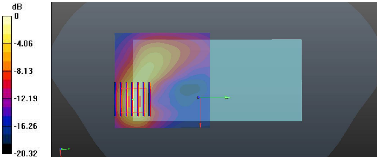
0 dB = 1.47 W/kg
