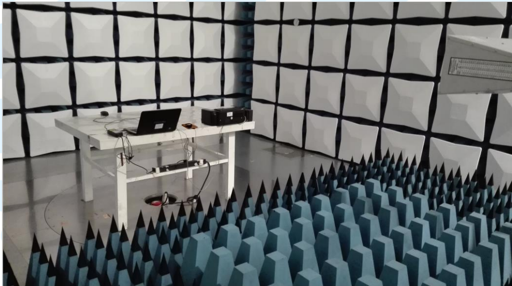
Radiated emission Test Setup-1(Above 1GHz)
