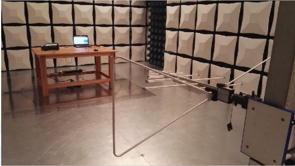
Radiated emission Test Setup-1(Below 1GHz)
