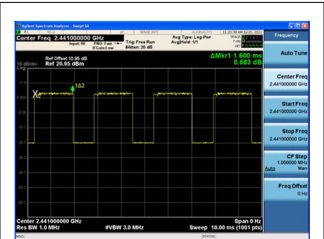
Modulation: 8DPSK 3DH3 2441
