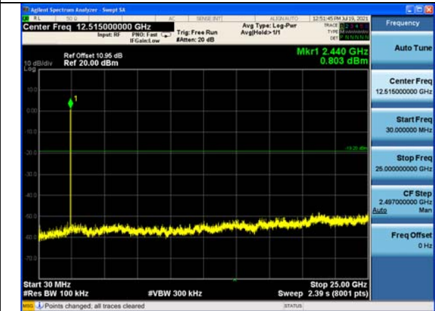
Test Mode:802.11b Chain0 CH6
