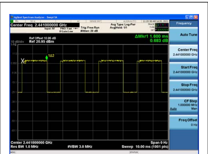
Modulation: 8DPSK 3DH3 2441
