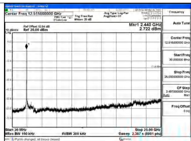
Test Mode:802.11n HT20 2437MHz Chain0
