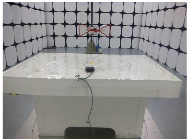
Radiated Spurious Emissions Test Setup 30MHz- 1GHz
