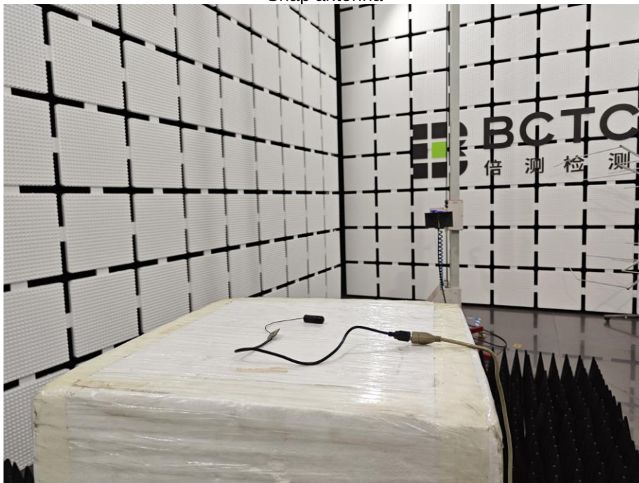
Snap antenna
