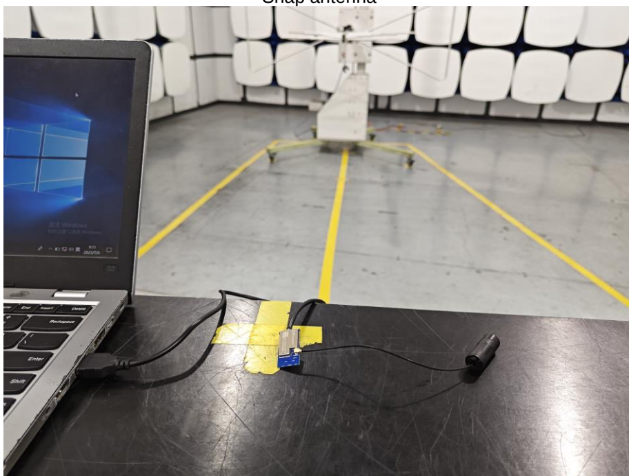
Snap antenna
