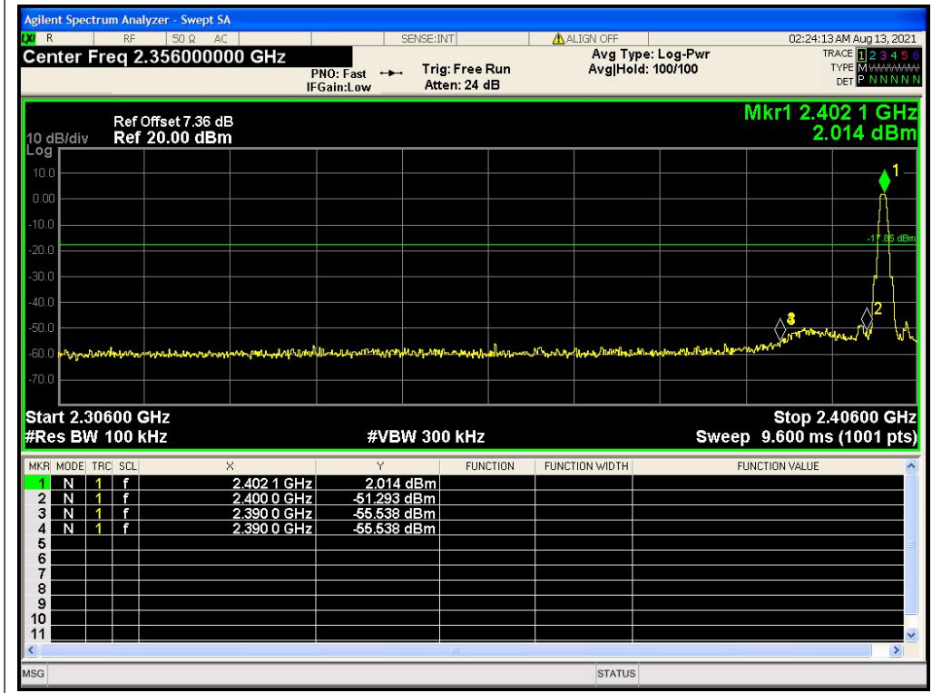
(LE 1M PHY _ Bandedge, Channel = 0)
