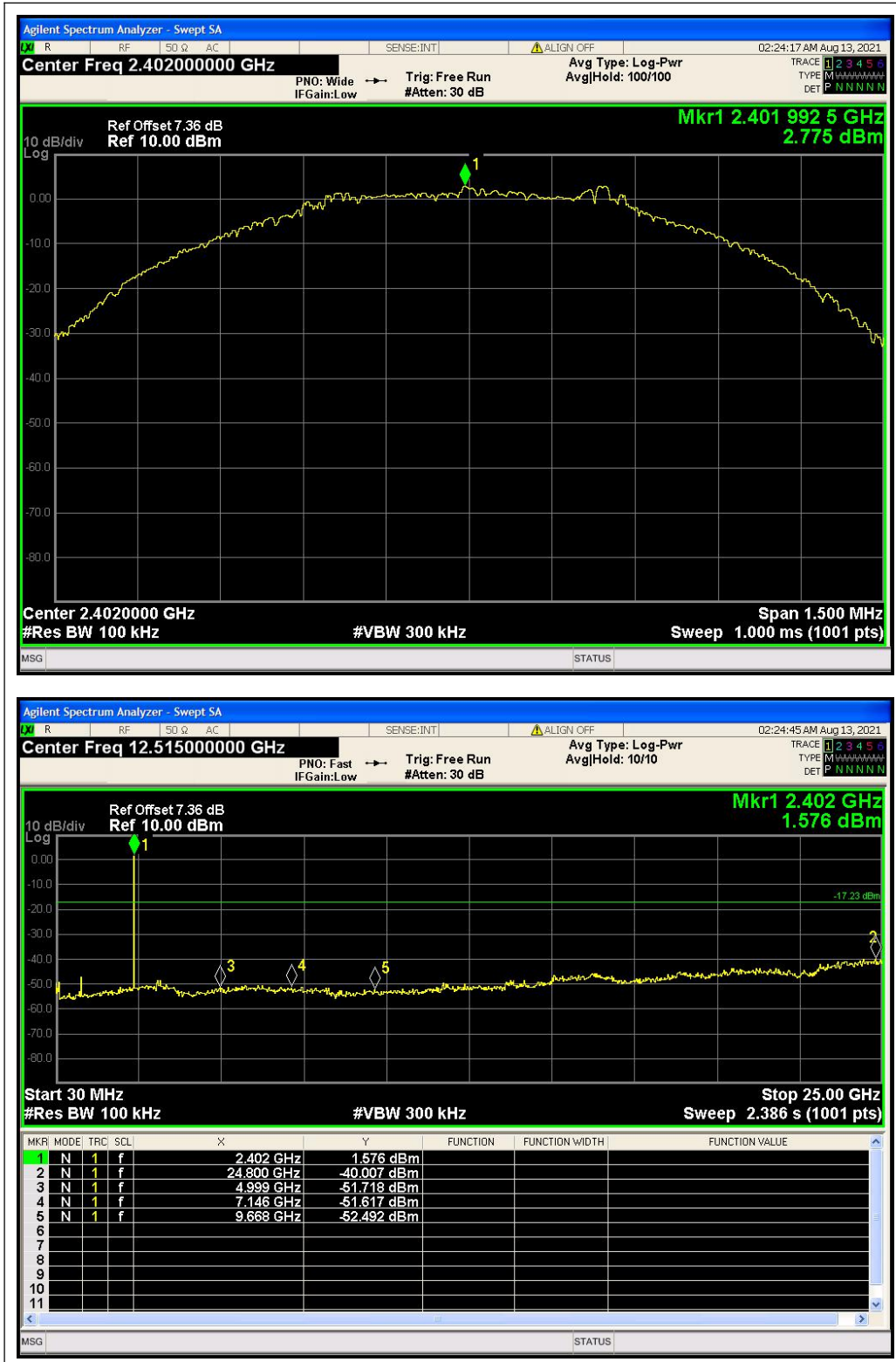
(LE 1M PHY _ Conducted Spurious Emissions _ Channel = 0, 30MHz to 25GHz)
