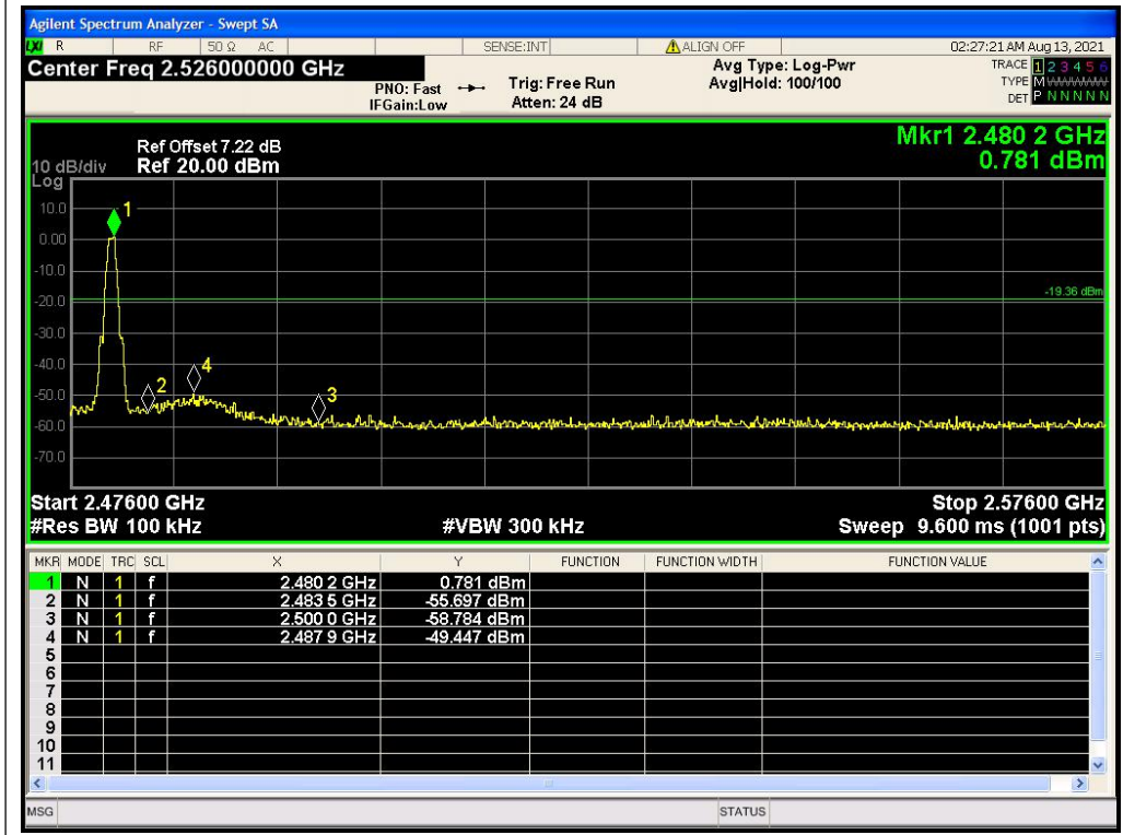
(LE 1M PHY _ Bandedge, Channel = 39)
