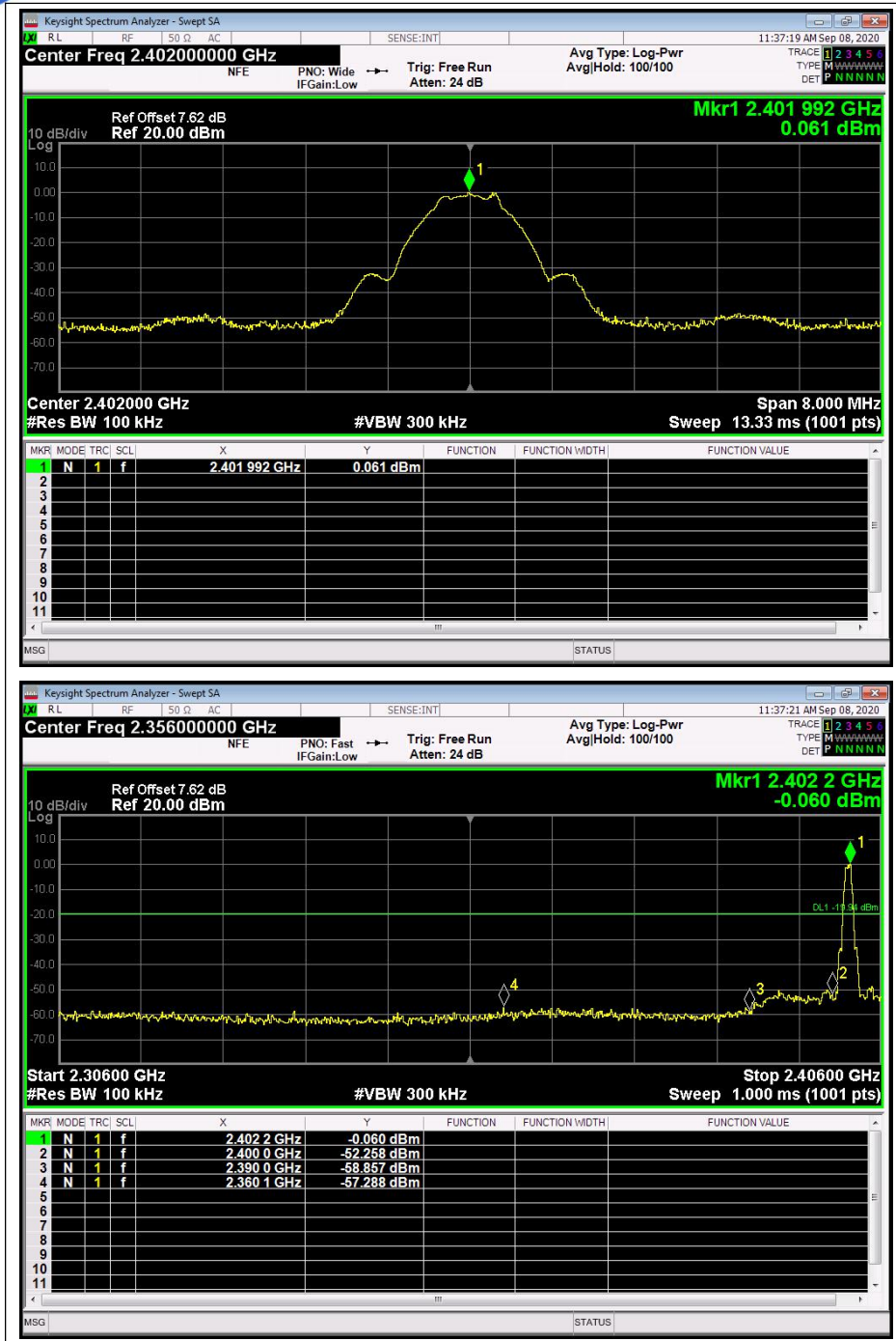
(Band Edge, Channel = 0)
