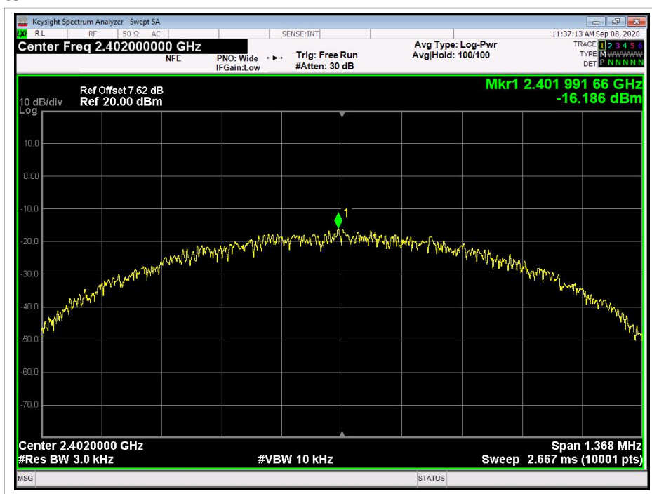
(Channel = 0, 2402MHz)
