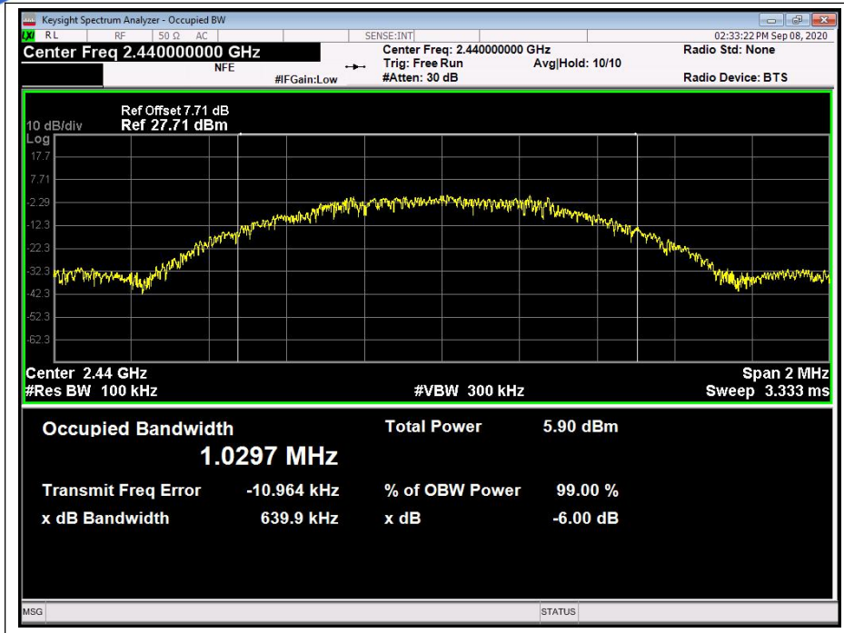
(Channel 19: 2440 MHz)
