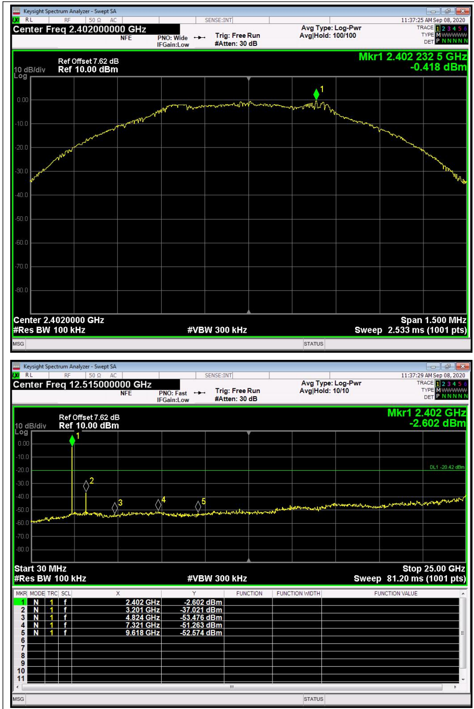
(Channel = 0, 30MHz to 25GHz)
