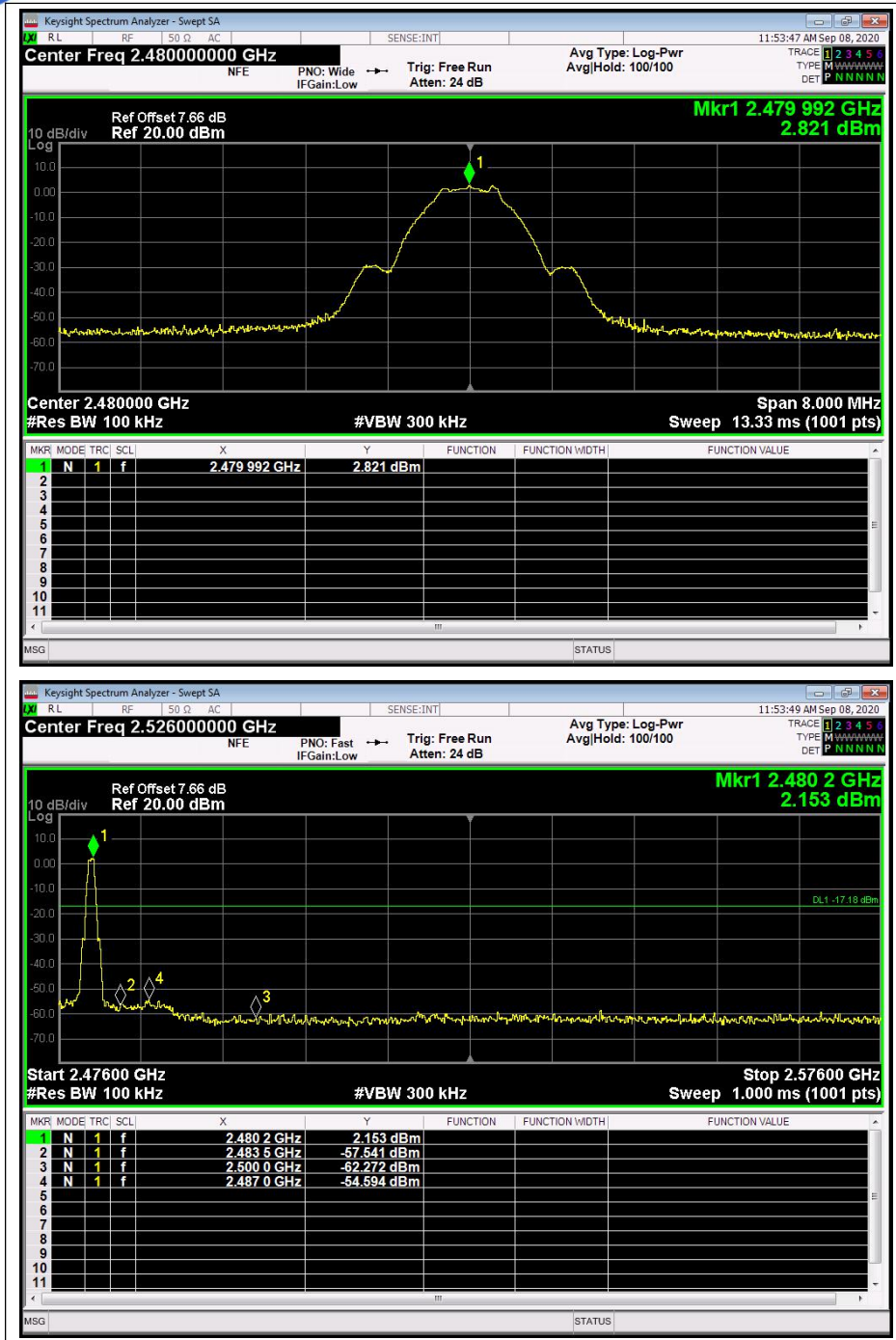
(Band Edge, Channel = 39)
