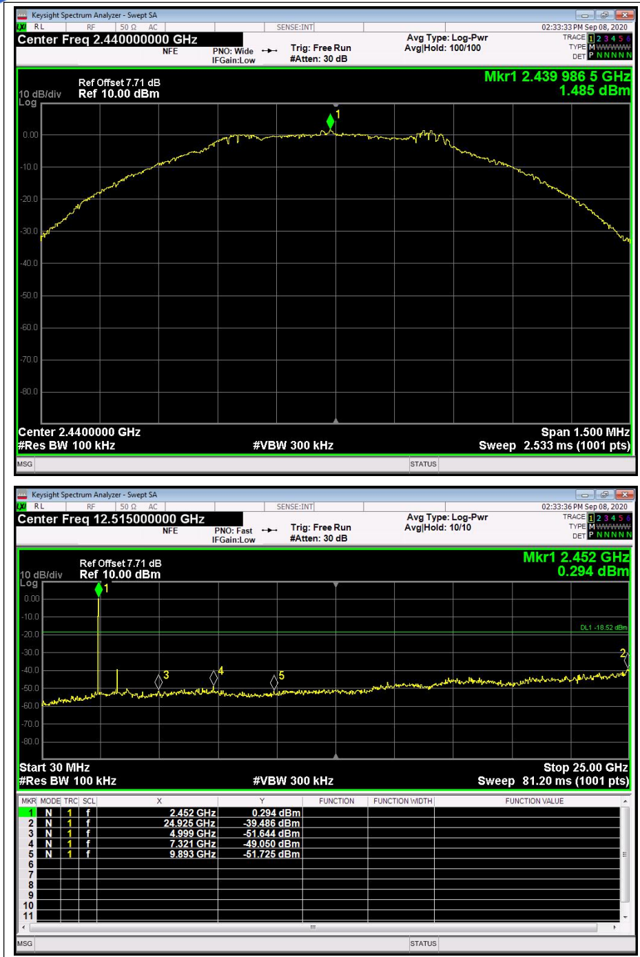
(Channel = 19, 30MHz to 25GHz)
