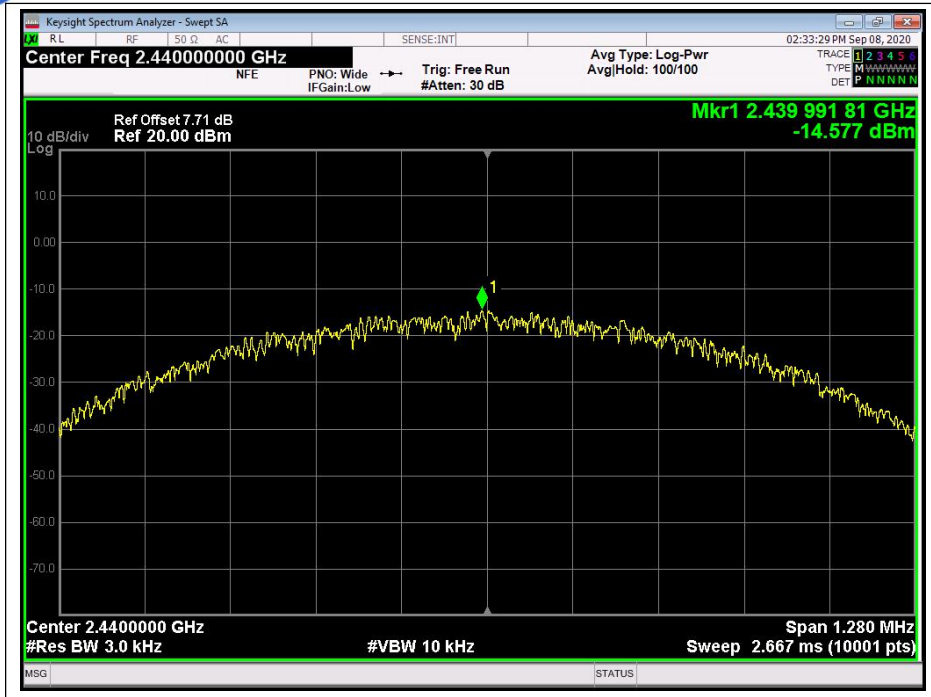
(Channel = 19, 2440MHz)
