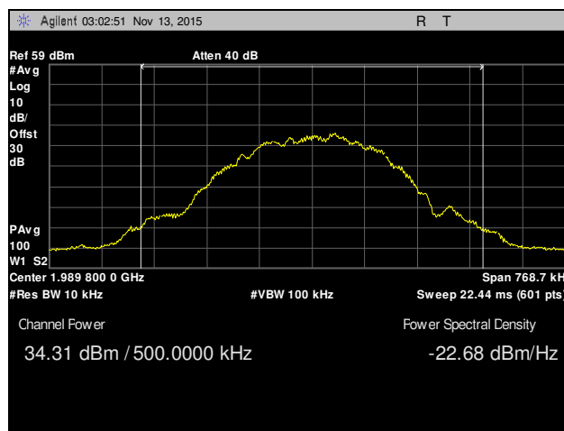
Plot 6, Channel 810, Conducted Power, Part 24
