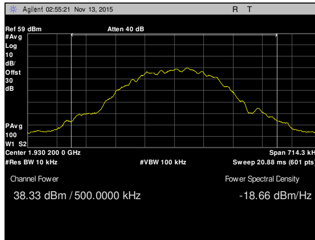
Plot 4, Channel 512, Conducted Power, Part 24
