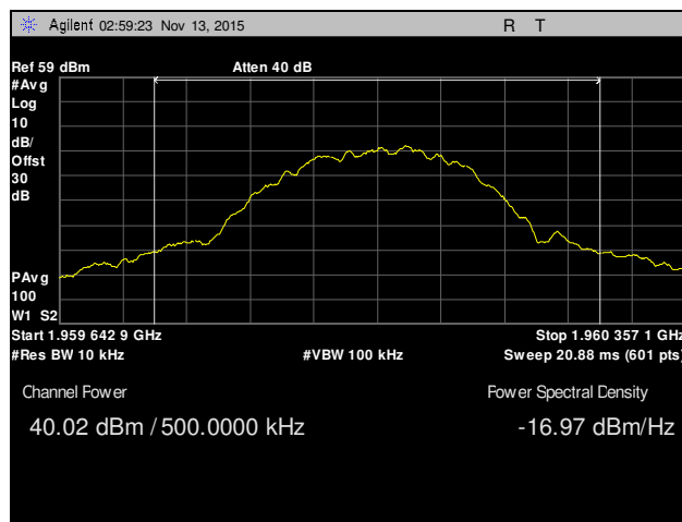
Plot 5, Channel 661, Conducted Power, Part 24
