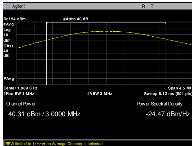
Plot 6. EIRP, Channel 1186, Conducted Power, Part 24
