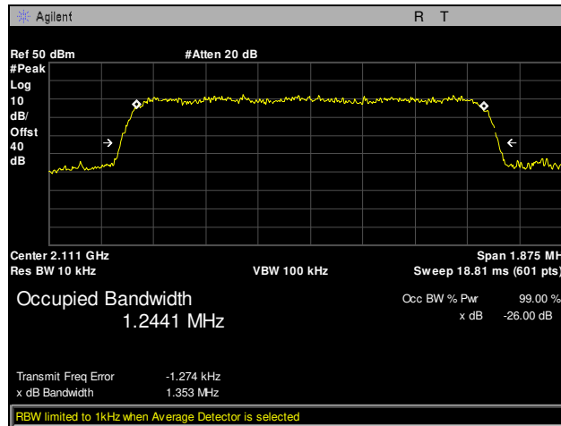
Plot 16. Occupied Bandwidth, Channel 14, Part 27
