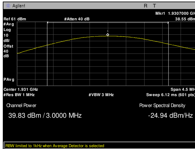
Plot 4. EIRP, Channel 14, Conducted Power, Part 24
