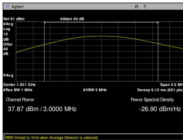
Plot 5. EIRP, Channel 425, Conducted Power, Part 24
