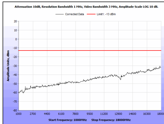
Plot 20. Radiated Spurious Emissions, Low Channel, 1 GHz – 18 GHz, Part 22
