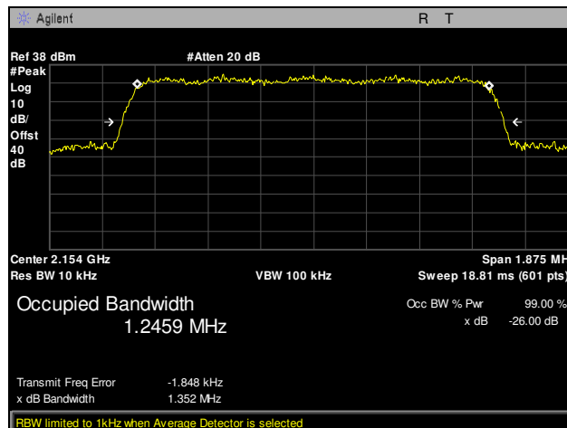
Plot 18. Occupied Bandwidth, Channel 886, Part 27
