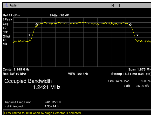
Plot 17. Occupied Bandwidth, Channel 700, Part 27
