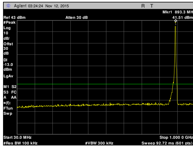
Plot 44. Conducted Spurious Emissions, Channel 4458, 30 MHz – 1 GHz, Part 22
