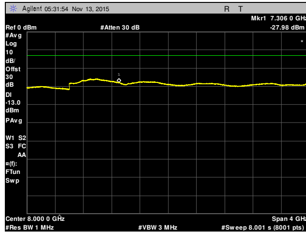
Plot 46. Conducted Spurious Emissions, Channel 4458, 6 GHz – 10 GHz, Part 22
