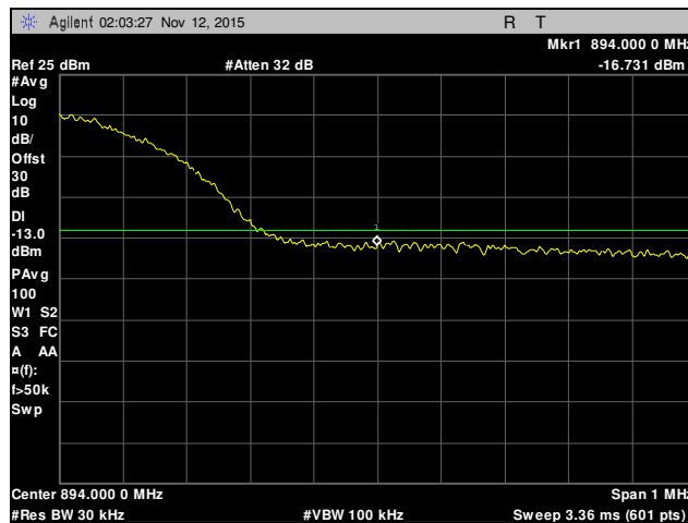
Plot 91. Conducted Band Edge, Channel 4457 (Full Power), Part 22
