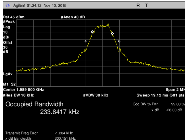
Plot 12. Occupied Bandwidth, Channel 810, Part 24
