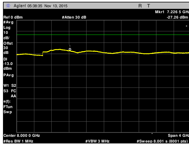
Plot 45. Conducted Spurious Emissions, Channel 661, 6 GHz – 10 GHz, Part 24
