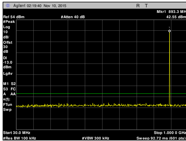
Plot 32. Conducted Spurious Emissions, Channel 251, 30 MHz – 1 GHz, Part 22
