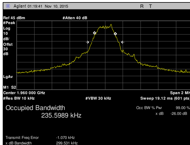
Plot 11. Occupied Bandwidth, Channel 661, Part 24
