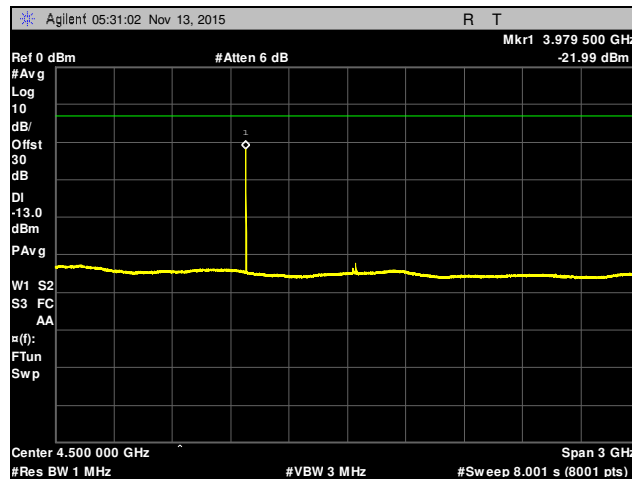
Plot 51. Conducted Spurious Emissions, Channel 810, 3 GHz – 6 GHz, Part 24
