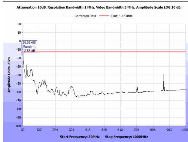
Plot 13. Radiated Spurious Emissions, Low Channel, 30 MHz – 1 GHz, Part 22
