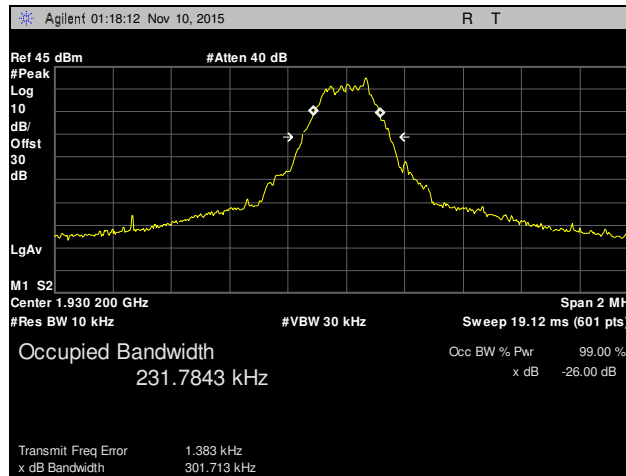
Plot 10. Occupied Bandwidth, Channel 512, Part 24
