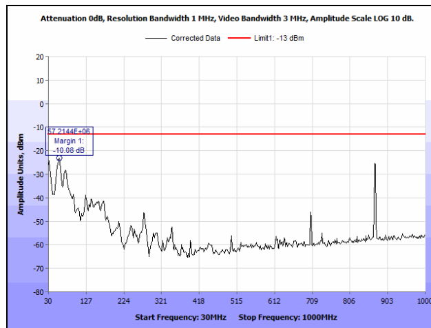
Plot 23. Radiated Spurious Emissions, High Channel, 30 MHz – 1 GHz, Part 22
