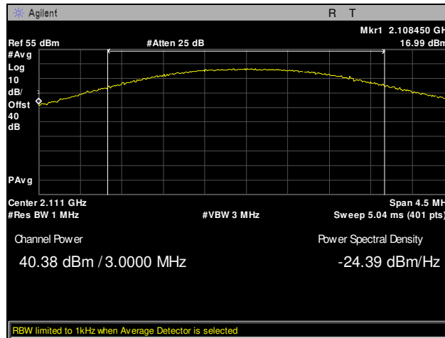
Plot 7. EIRP, Channel 14, Conducted Power, Part 27
