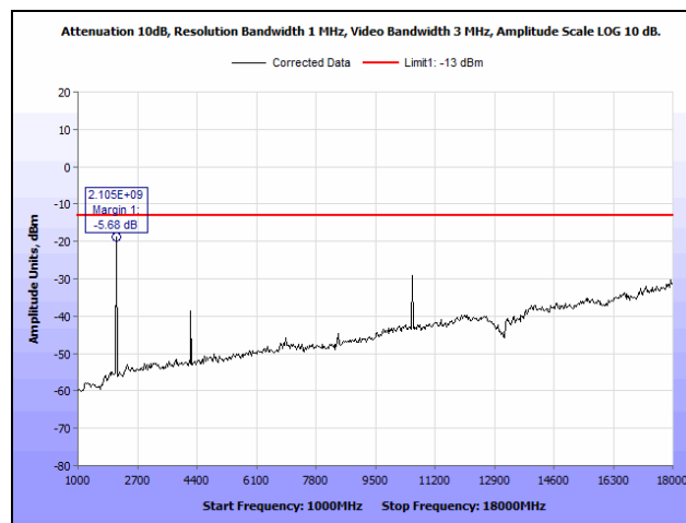
Plot 32. Radiated Spurious Emissions, Low Channel, 1 GHz – 18 GHz, Part 27
