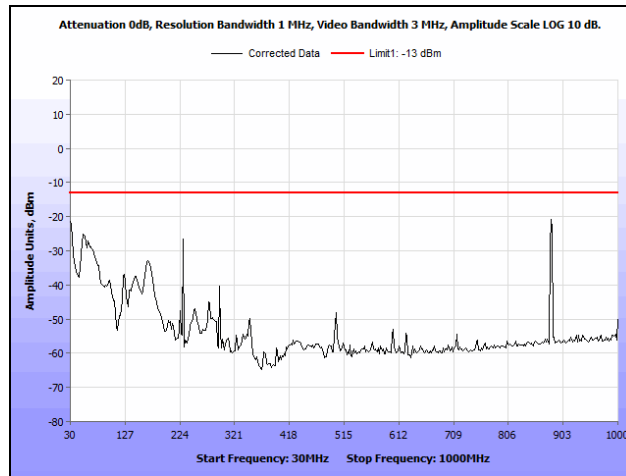
Plot 19. Radiated Spurious Emissions, Low Channel, 30 MHz – 1 GHz, Part 22
