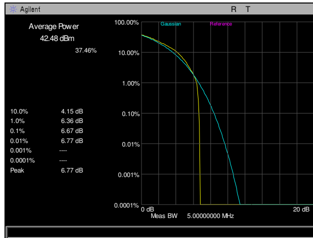
Plot 99. Peak to Average Ratio, Channel 356, Part 22
