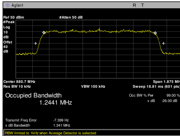
Plot 10. Occupied Bandwidth, Channel 356, Part 22
