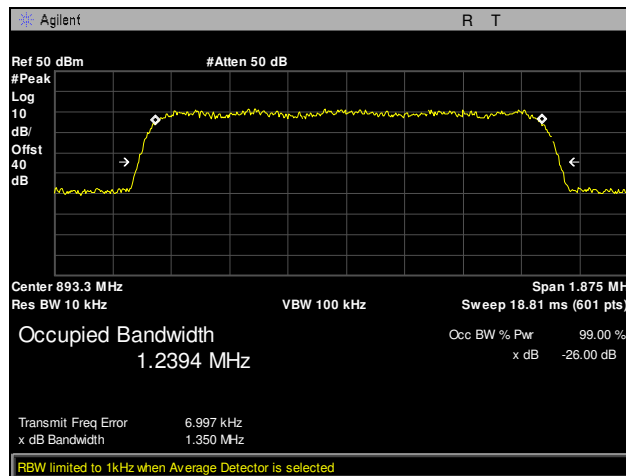
Plot 11. Occupied Bandwidth, Channel 777, Part 22
