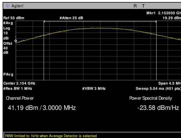
Plot 9. EIRP, Channel 886, Conducted Power, Part 27
