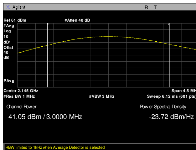
Plot 8. EIRP, Channel 700, Conducted Power, Part 27
