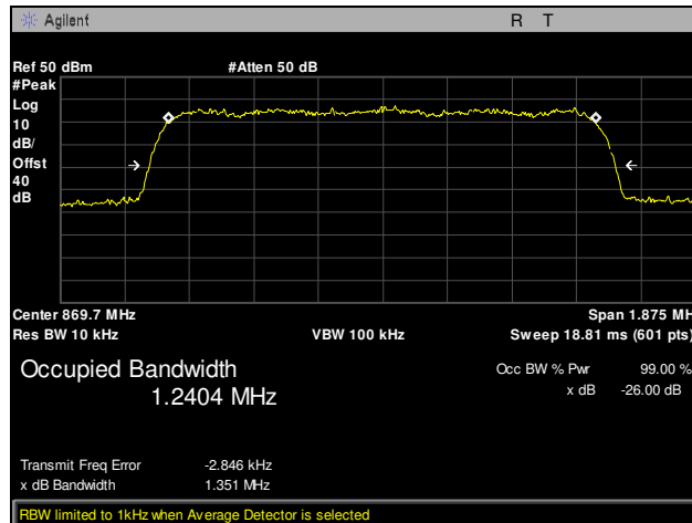
Plot 12. Occupied Bandwidth, Channel 1013, Part 22
