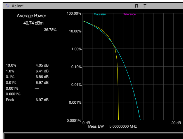
Plot 100. Peak to Average Ratio, Channel 777, Part 22
