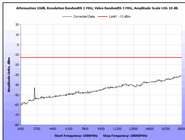
Plot 24. Radiated Spurious Emissions, High Channel, 1 GHz – 18 GHz, Part 22
