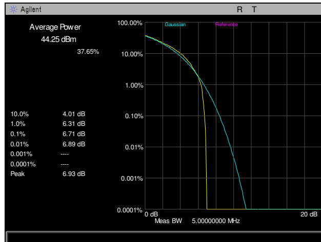
Plot 101. Peak to Average Ratio, Channel 1013, Part 22
