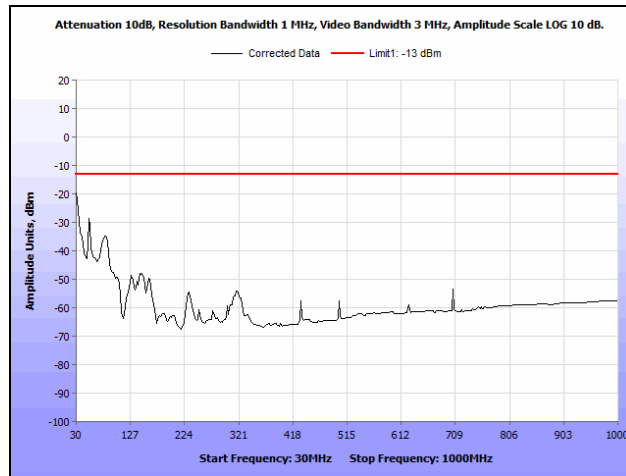
Plot 25. Radiated Spurious Emissions, Low Channel, 30 MHz – 1 GHz, Part 24
