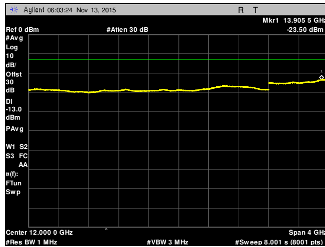
Plot 51. Conducted Spurious Emissions, Channel 6592, 10 GHz – 14 GHz, Part 24
