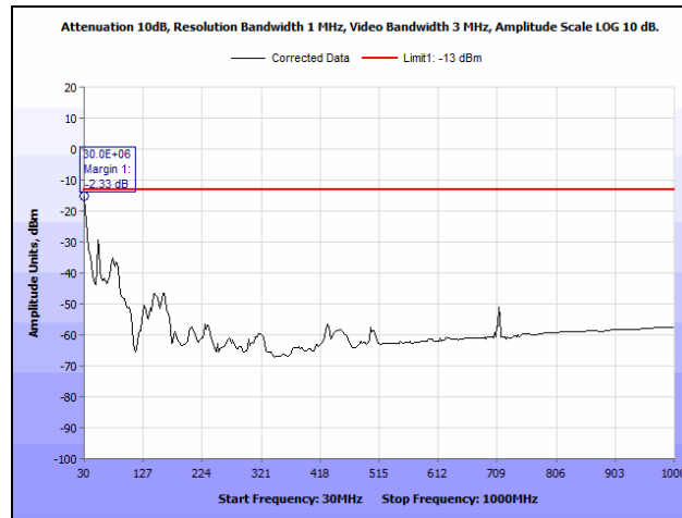
Plot 31. Radiated Spurious Emissions, Low Channel, 30 MHz – 1 GHz, Part 27
