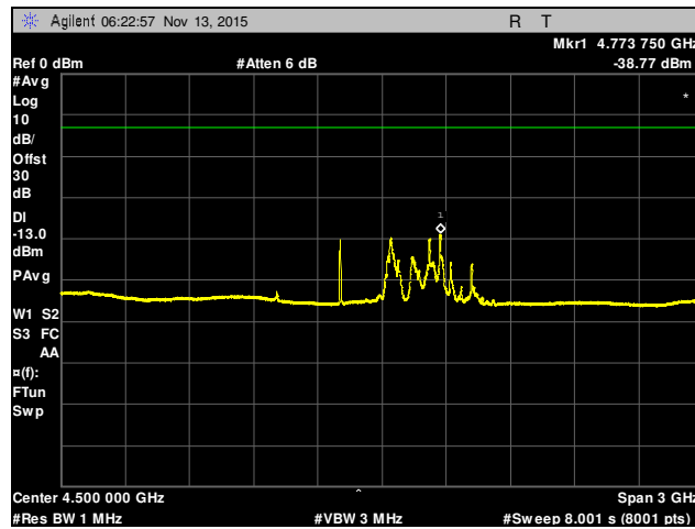
Plot 84. Conducted Spurious Emissions, Channel 2087, 3 GHz – 6 GHz, Part 27
