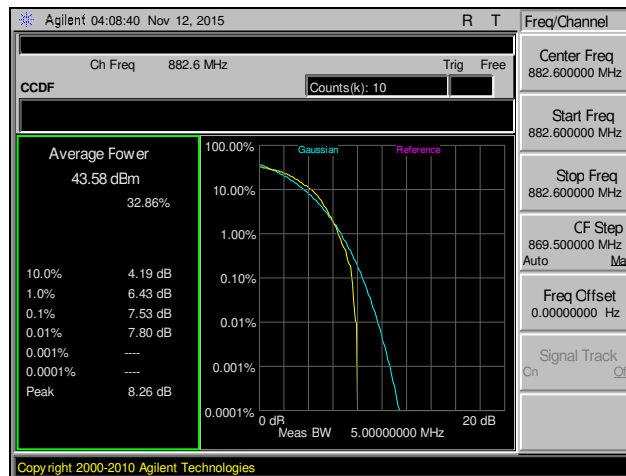
Plot 101. Peak to Average Ratio, Channel 4413, Part 22
