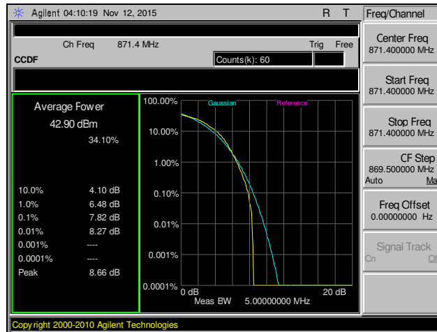
Plot 100. Peak to Average Ratio, Channel 4357, Part 22
