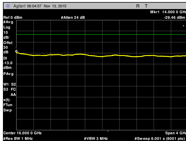
Plot 52. Conducted Spurious Emissions, Channel 6592, 14 GHz – 18 GHz, Part 24
