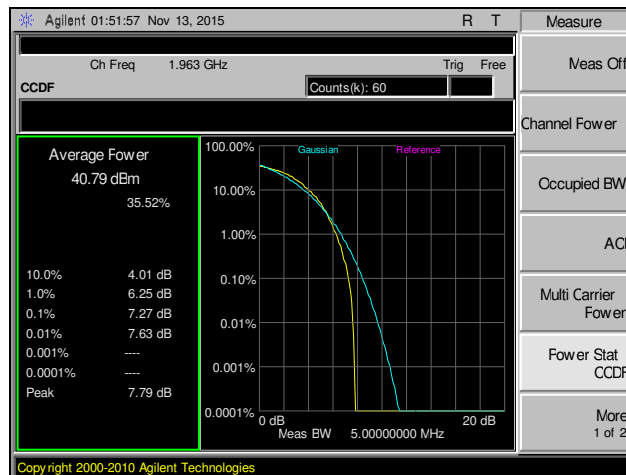
Plot 105. Peak to Average Ratio, Channel 9815, Part 24
