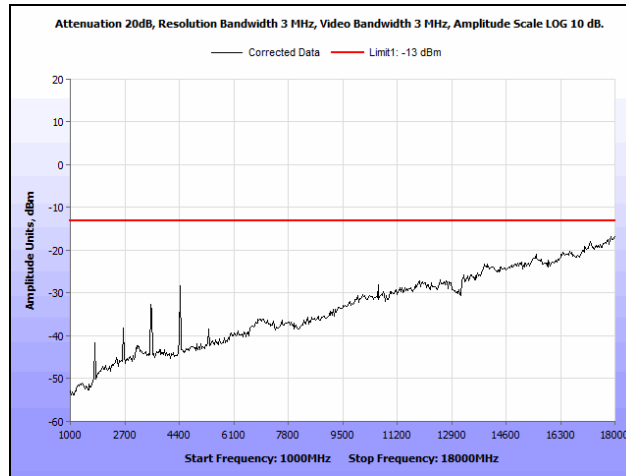
Plot 22. Radiated Spurious Emissions, Mid Channel, 1 GHz – 18 GHz, Part 22
