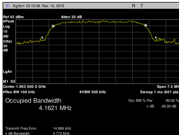
Plot 15. Occupied Bandwidth, Channel 9815, Part 24
