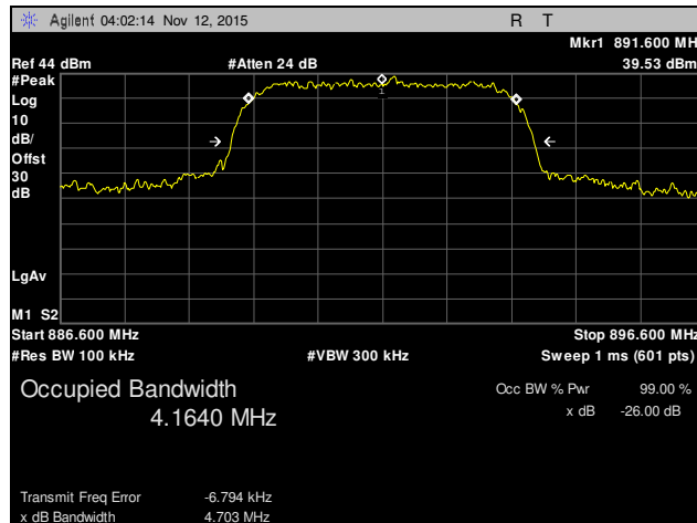
Plot 12. Occupied Bandwidth, Channel 4458, Part 22
