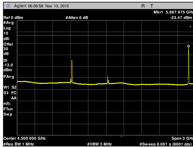
Plot 63. Conducted Spurious Emissions, Channel 9815, 3 GHz – 6 GHz, Part 24
