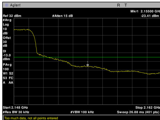
Plot 98. Conducted Band Edge, Channel 2062 (Full Power), Part 27
