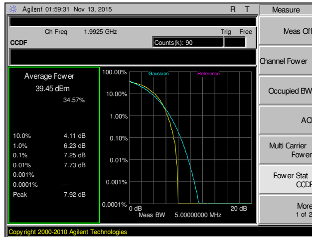
Plot 103. Peak to Average Ratio, Channel 6592, Part 24
