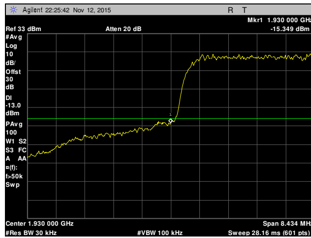
Plot 94. Conducted Band Edge, Channel 5513 (Full Power), Part 24
