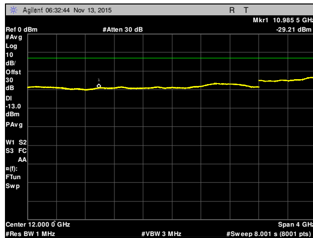
Plot 79. Conducted Spurious Emissions, Channel 1655, 10 GHz – 14 GHz, Part 27
