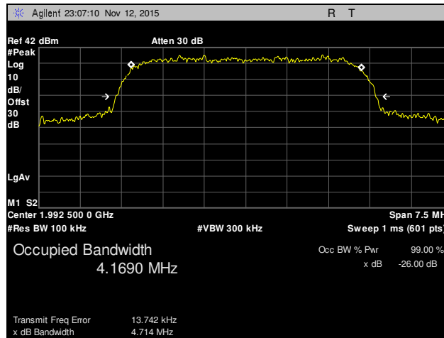
Plot 13. Occupied Bandwidth, Channel 6592, Part 24
