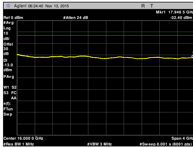
Plot 87. Conducted Spurious Emissions, Channel 2087, 14 GHz – 18 GHz, Part 27
