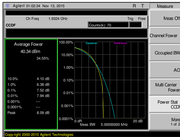
Plot 104. Peak to Average Ratio, Channel 9662, Part 24
