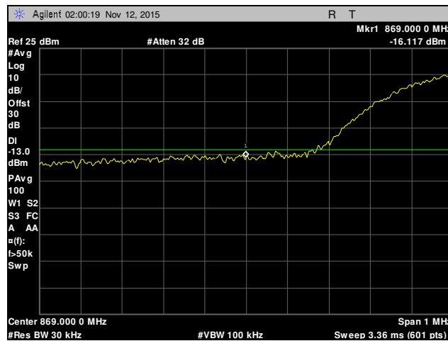
Plot 90. Conducted Band Edge, Channel 4358 (Full Power), Part 22
