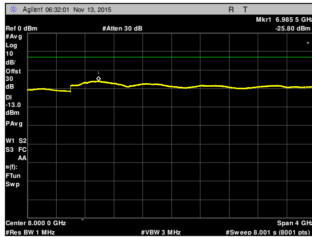
Plot 78. Conducted Spurious Emissions, Channel 1655, 6 GHz – 10 GHz, Part 27
