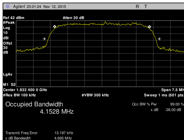
Plot 14. Occupied Bandwidth, Channel 9662, Part 24
