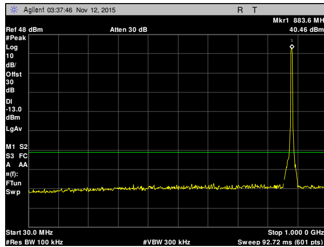
Plot 41. Conducted Spurious Emissions, Channel 4413, 30 MHz – 1 GHz, Part 22
