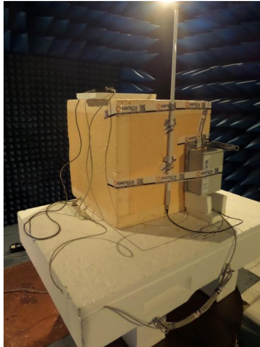
Anechoic chamber setup 6dBi antenna
