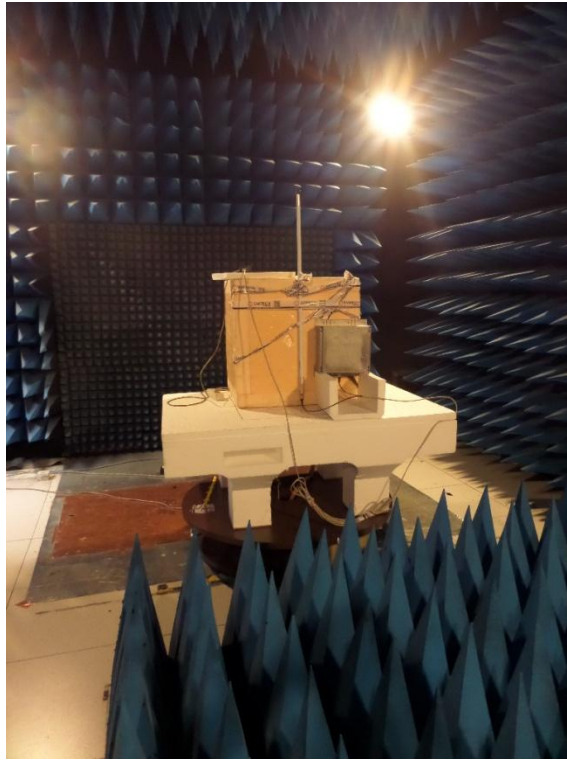
Anechoic chamber setup 6dBi antenna
