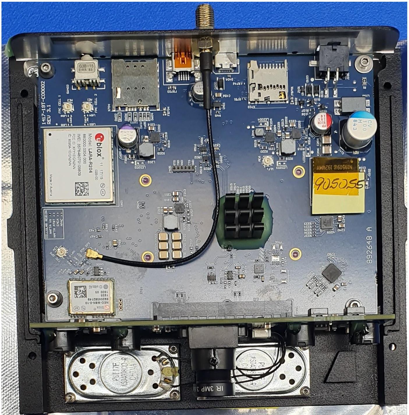
Figure 8 OAS-LV 204 Top Cover Removed
