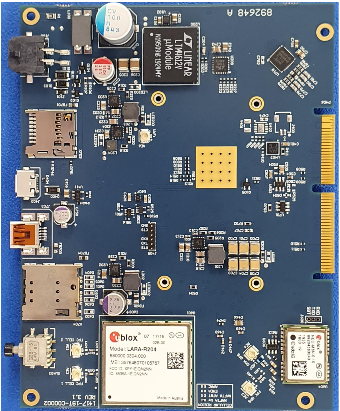
Figure 10 905055 PCBA, Carrier Board CPU AT&T PCB Top View
