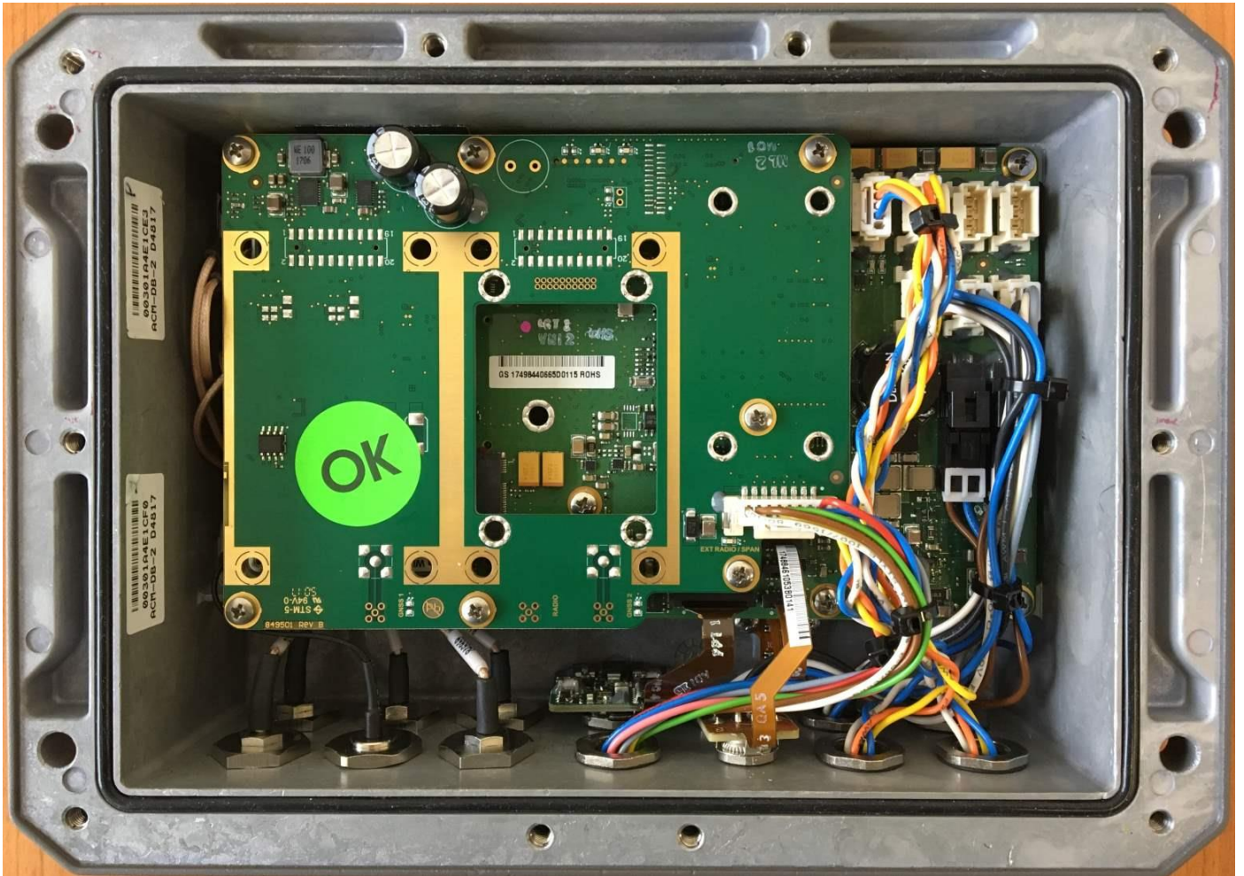
Figure 10 CoreLP Bottom Cover Removed
