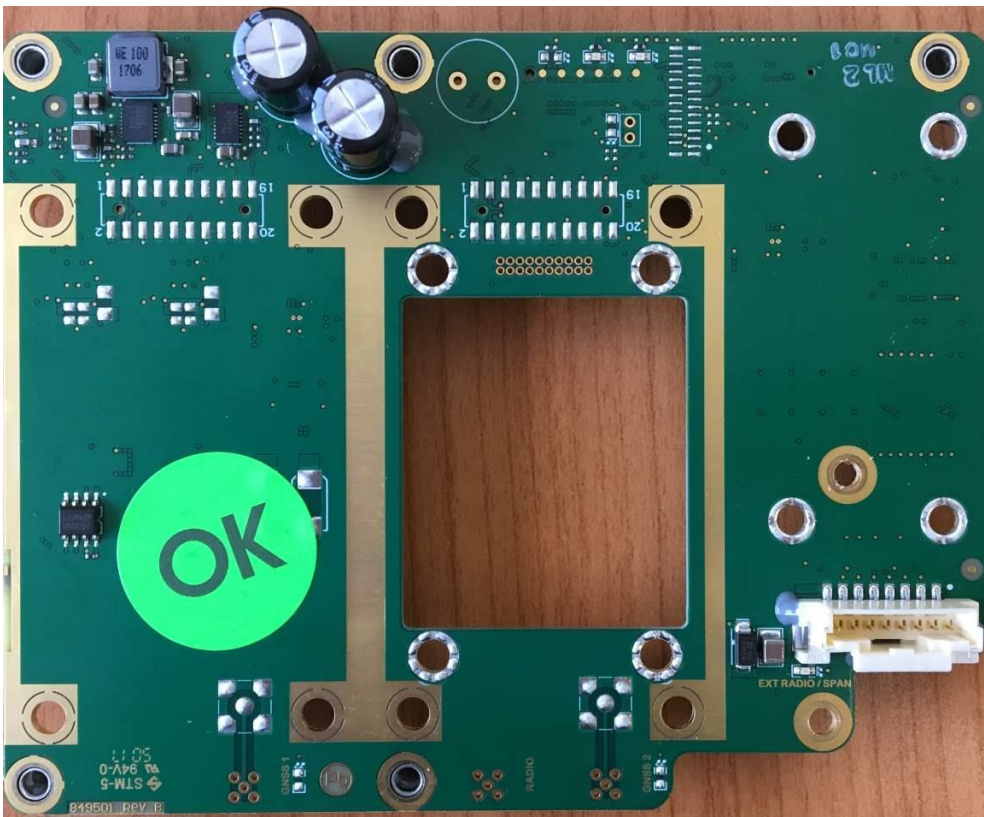
Figure 16 Blackwidow PCB Top View
