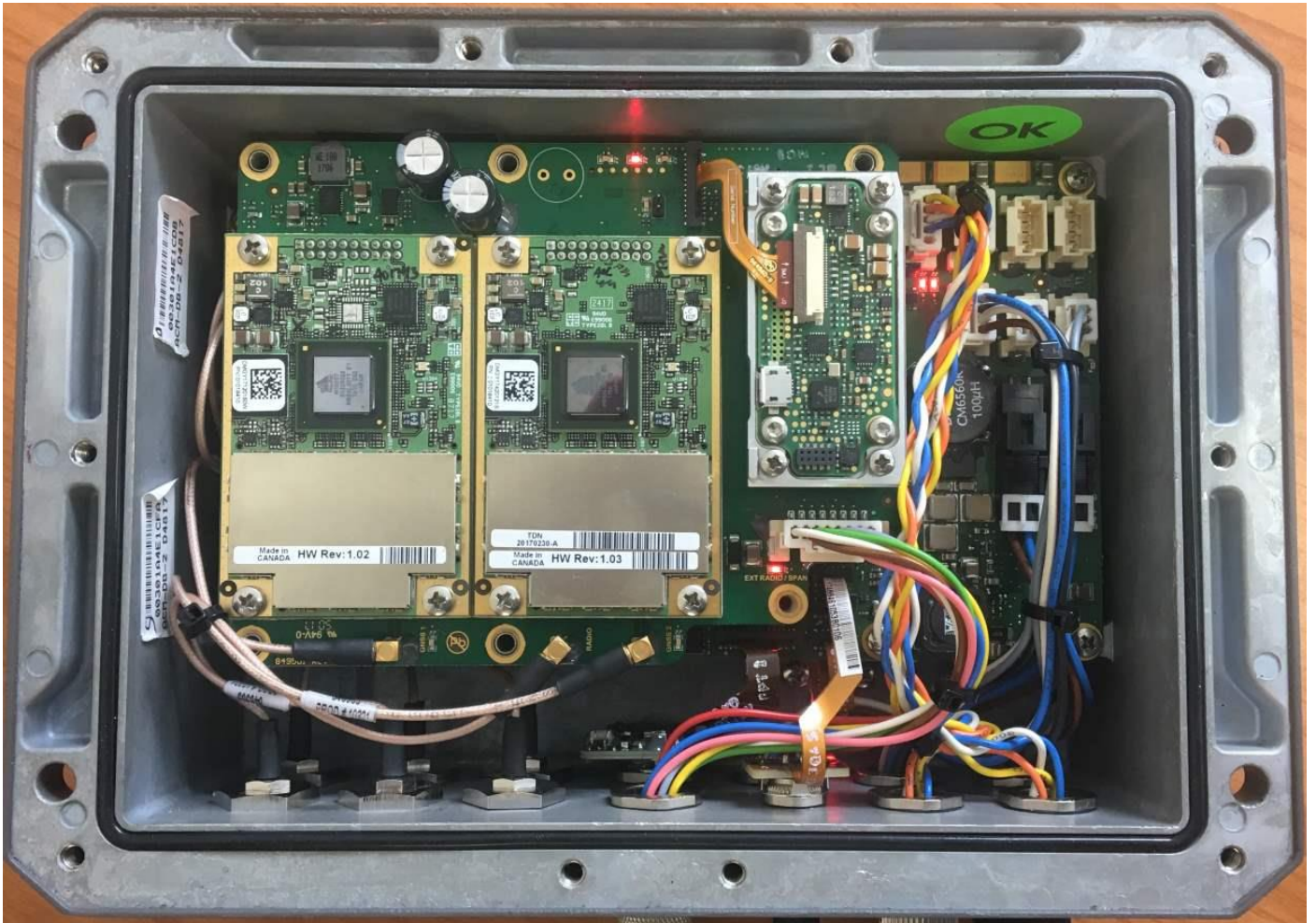
Figure 5 Core HP Bottom Cover Removed
