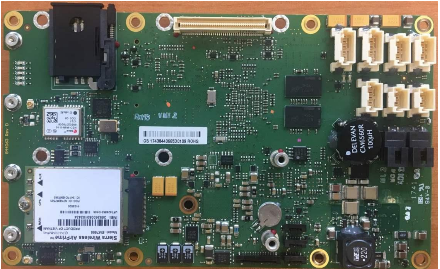
Figure 12 ARC Reactor Top View with Optional 4G Module
