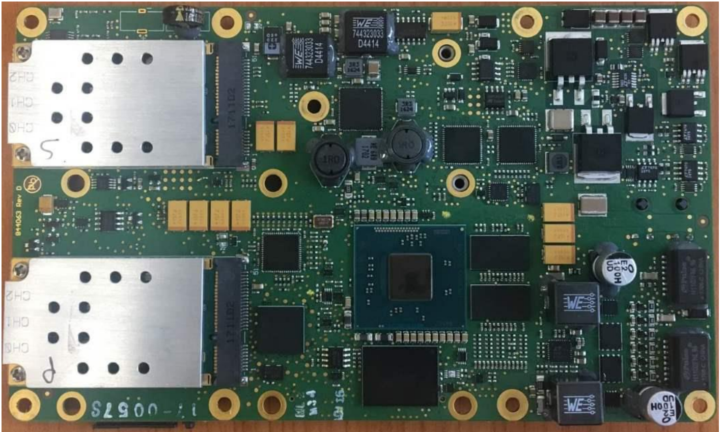
Figure 13 ARC Reactor PCB Bottom View with WiFi Modules
