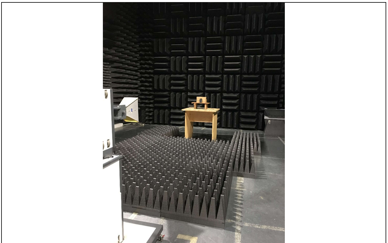
Photograph 3: photo of the EUT tested in the range 1000-12750 MHz with Horn Antenna
