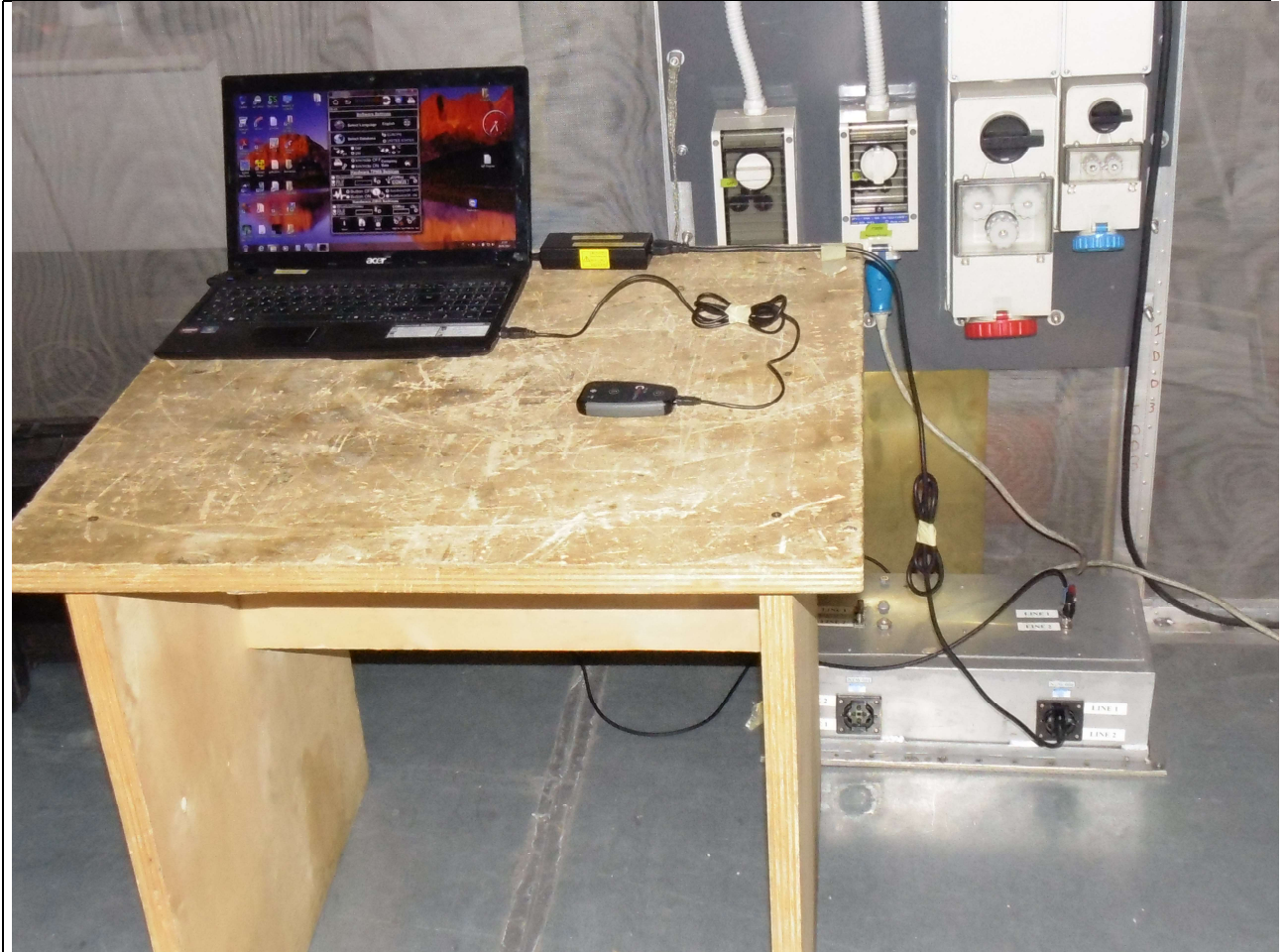
Photograph 4: photo of the EUT in the AC Mains Conducted Emission test
