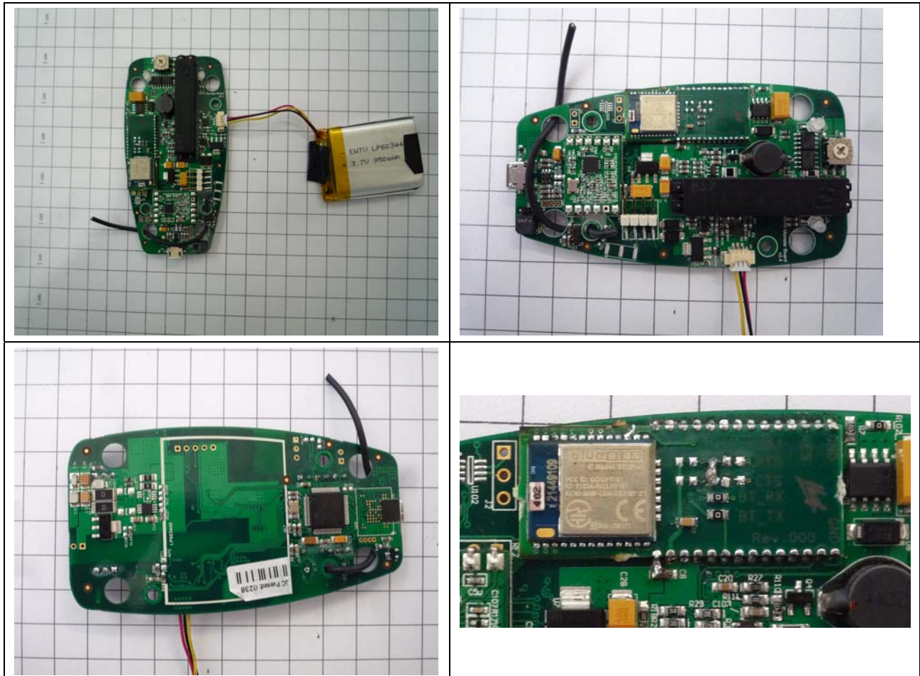
Photograph 3: EUT identification – internal view
