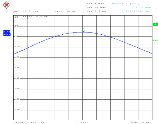
Lowest channel
