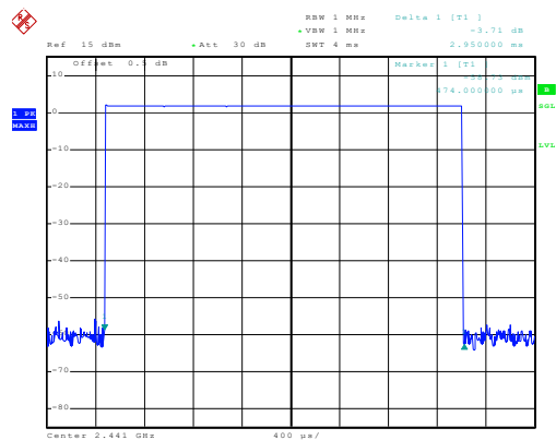
DH5/2-DH5/3-DH5
