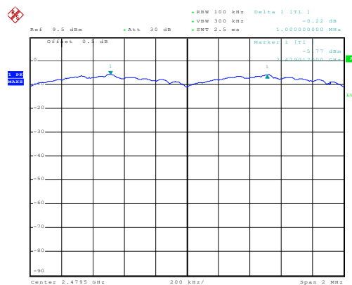
Highest channel
