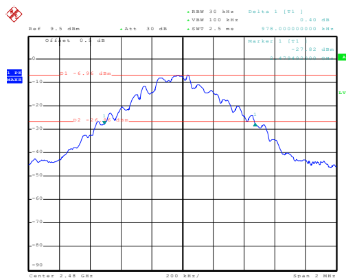
Highest channel
