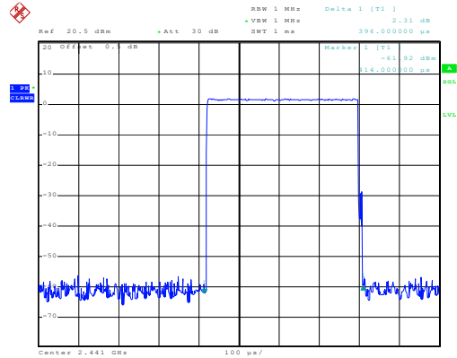
DH1/2-DH1/3-DH1
