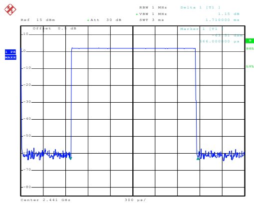
DH3/2-DH3/3-DH3
