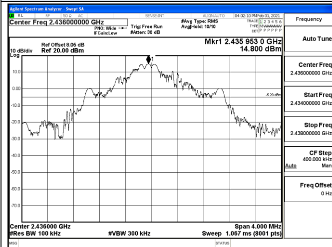
Channel 7 / 2436 MHz
