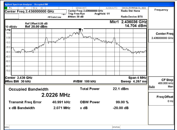
Channel 7/2436Hz
