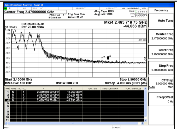
Channel 15 / 2460 MHz
