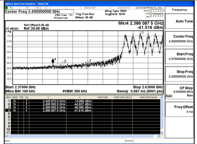
Channel 0 / 2415 MHz
