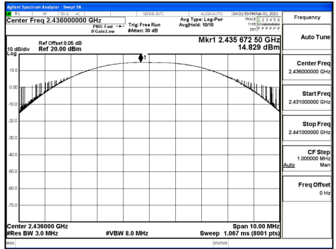
Channel 7 / 2436MHz
