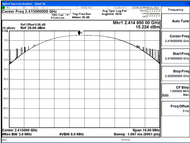
Channel 0 / 2415 MHz
