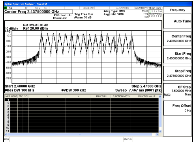
Channel 7 / 2436 MHz
