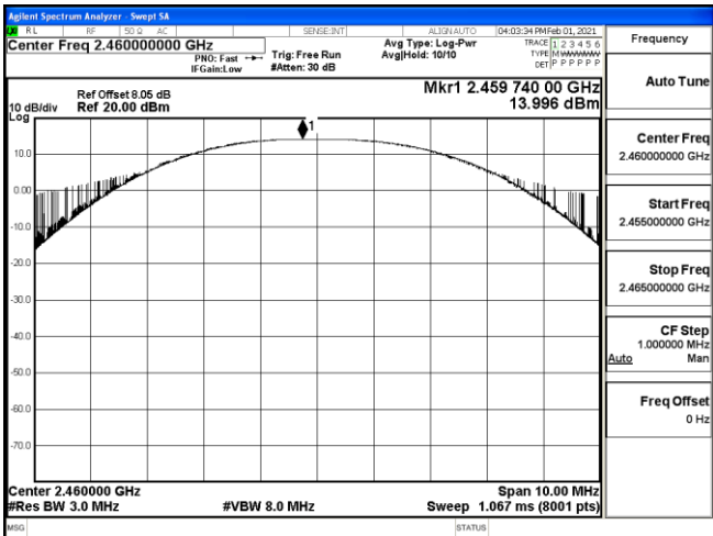
Channel 15 / 2460 MHz
