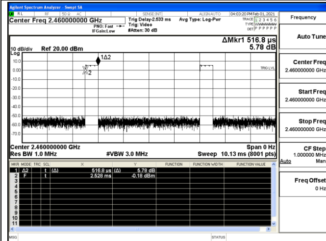
Channel 15/ 2460 MHz
