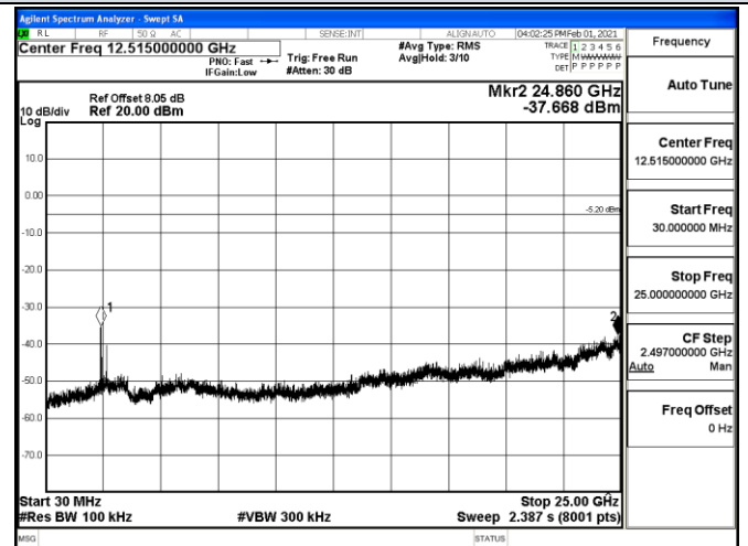
Channel 7 / 2436 MHz
