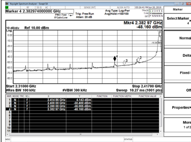
Channel 0 / 2415 MHz
