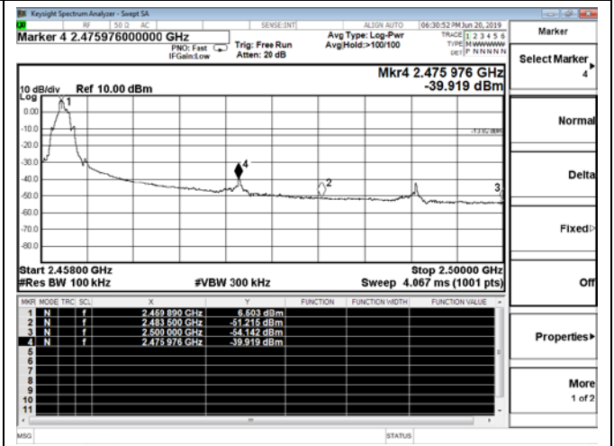
Channel 15 / 2460 MHz
