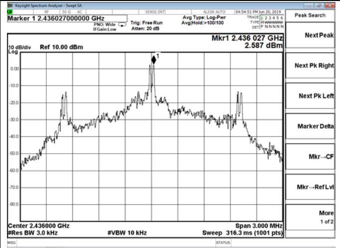
Channel 7 / 2436 MHz
