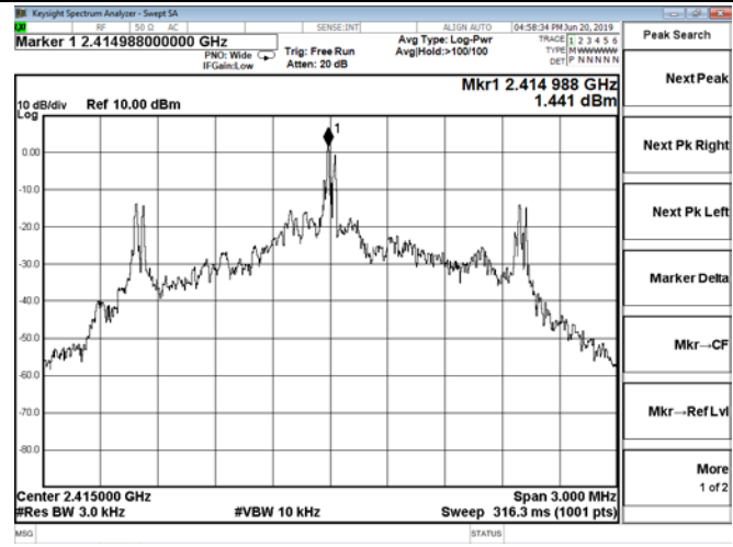
Channel 0 / 2415 MHz
