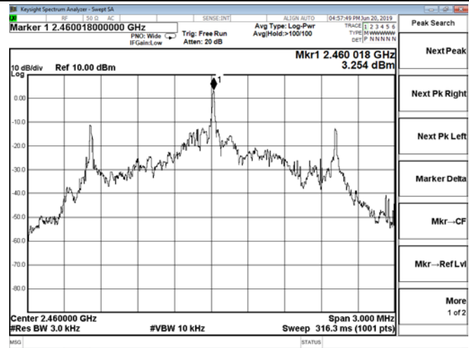
Channel 15 / 2460 MHz
