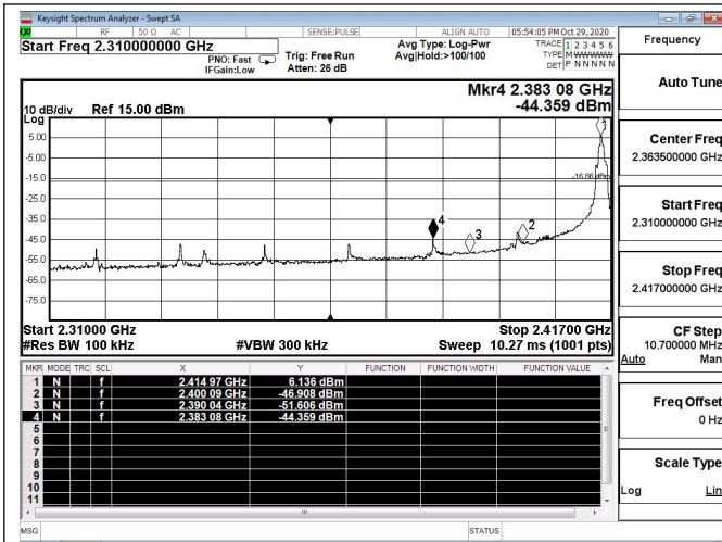
Channel 0 / 2415 MHz
