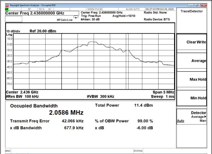
Channel 7/ 2436Hz
