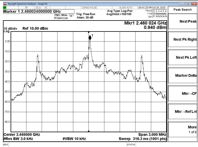
Channel 15/ 2460 MHz
