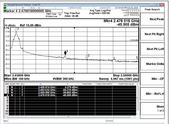
Channel 15 / 2460 MHz
