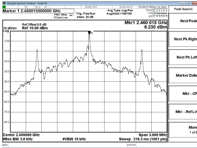
Channel 15/ 2460 MHz
