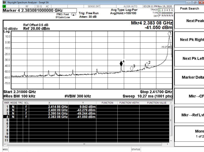
Channel 0 / 2415 MHz
