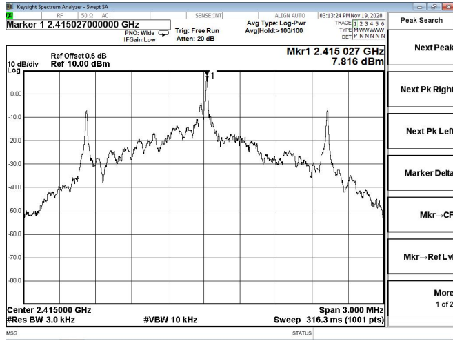
Channel 0 / 2415 MHz
