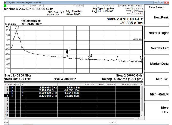
Channel 15 / 2460 MHz
