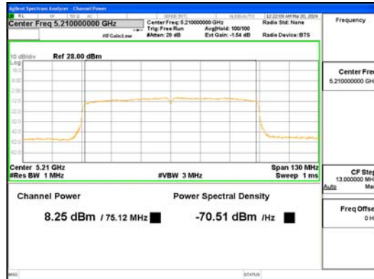
802.11ac_VHT80_UNII 1
