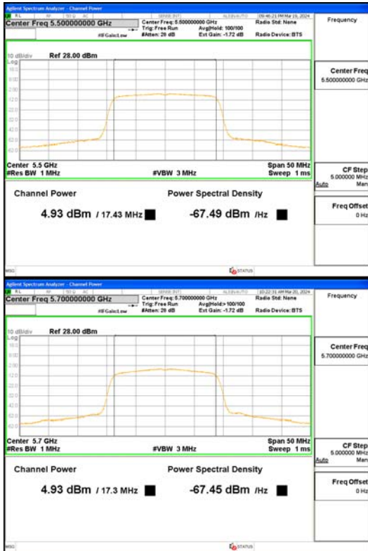
802.11ac_VHT20_UNII 2C
