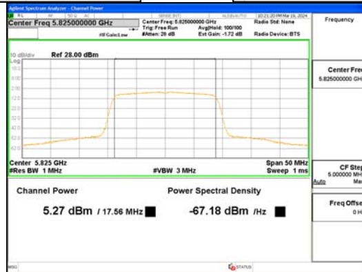
802.11ac_VHT20_UNII 3
