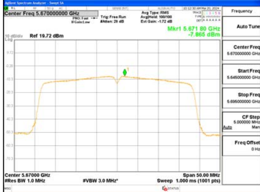
802.11n_HT40_UNII 2C
