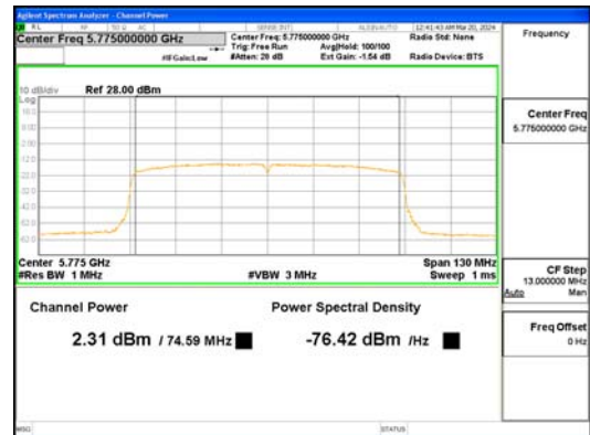
802.11ac_VHT80_UNII 3
