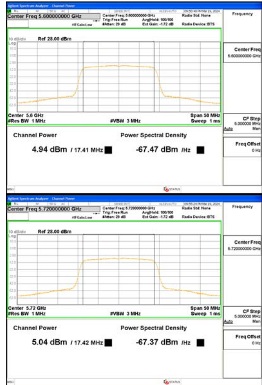
802.11ac_VHT20_UNII 2C
