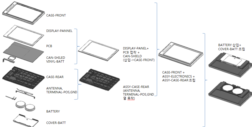
Figure 4 Exploded View
