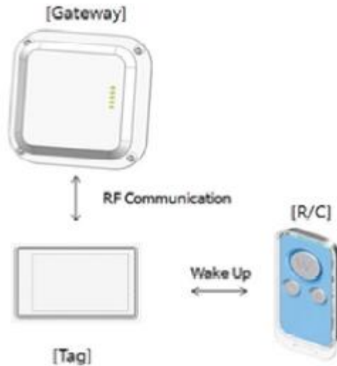
Figure 6 Operation Test
