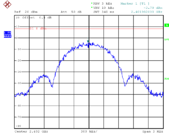
Test Mode : ANT2 Low channel
