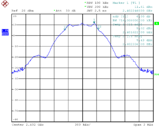
6 dB Bandwidth[MHz] Low channel
