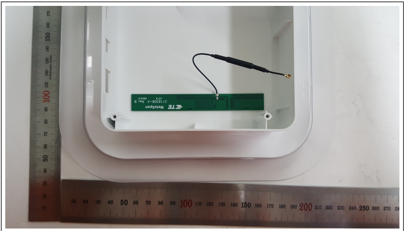
< Antenna >
