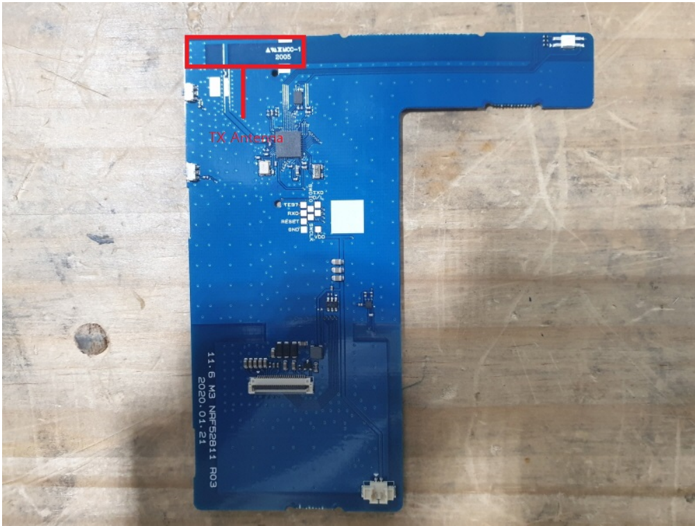
TX Antenna
