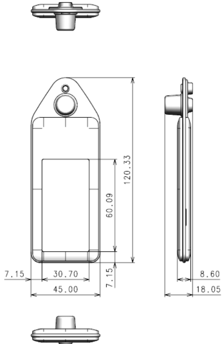
Figure 3 Mechanical Dimension
