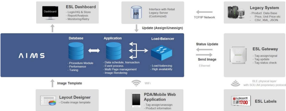
Figure 1. ESL System
