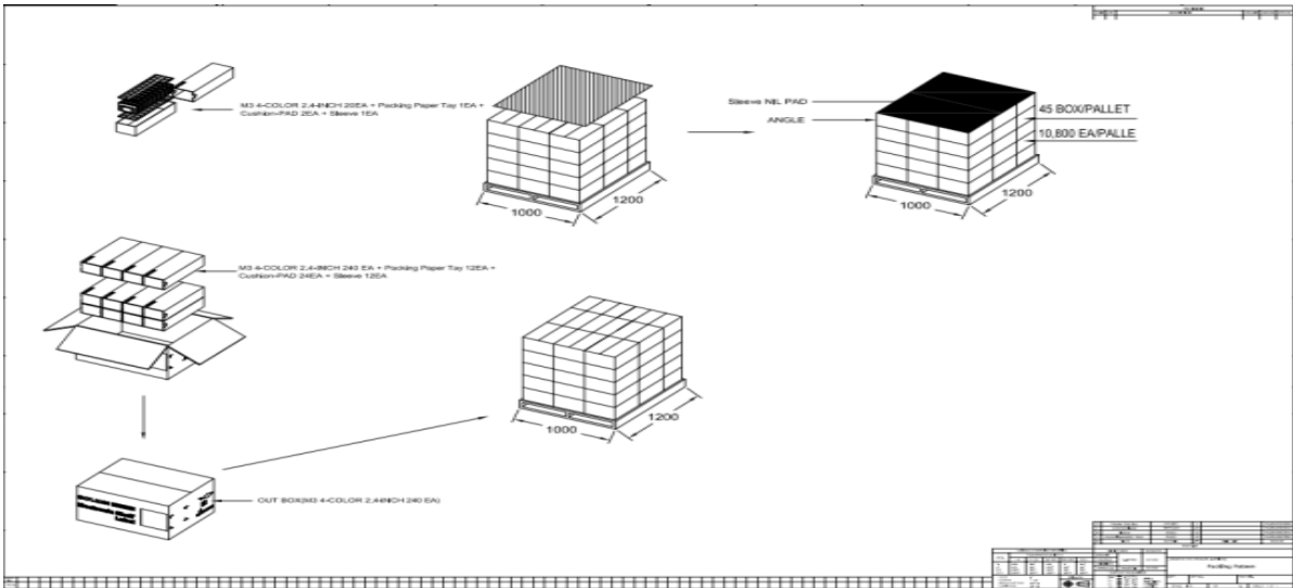
Figure 14. Package
