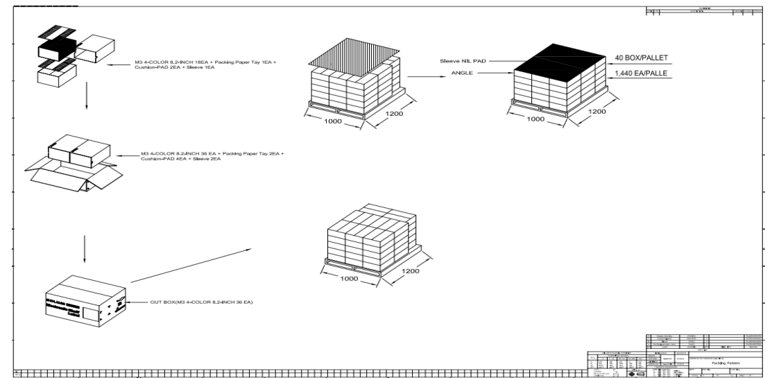
Figure 14. Package
