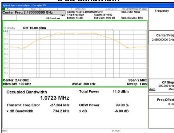
6 dB Bandwidth
