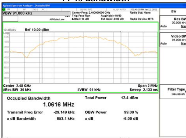
99 % Bandwidth
