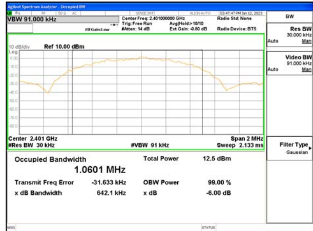
99 % Bandwidth
