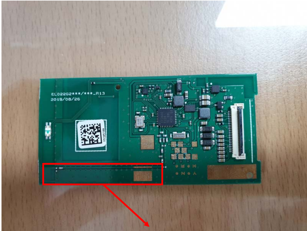
Wake up Antenna (RX)
