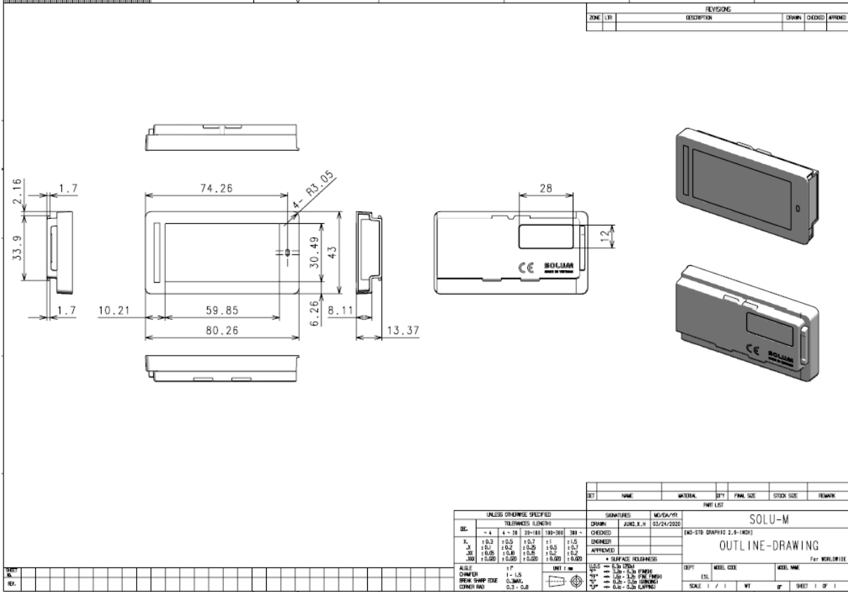
Figure 5. 2.6" Mechanical Dimension
