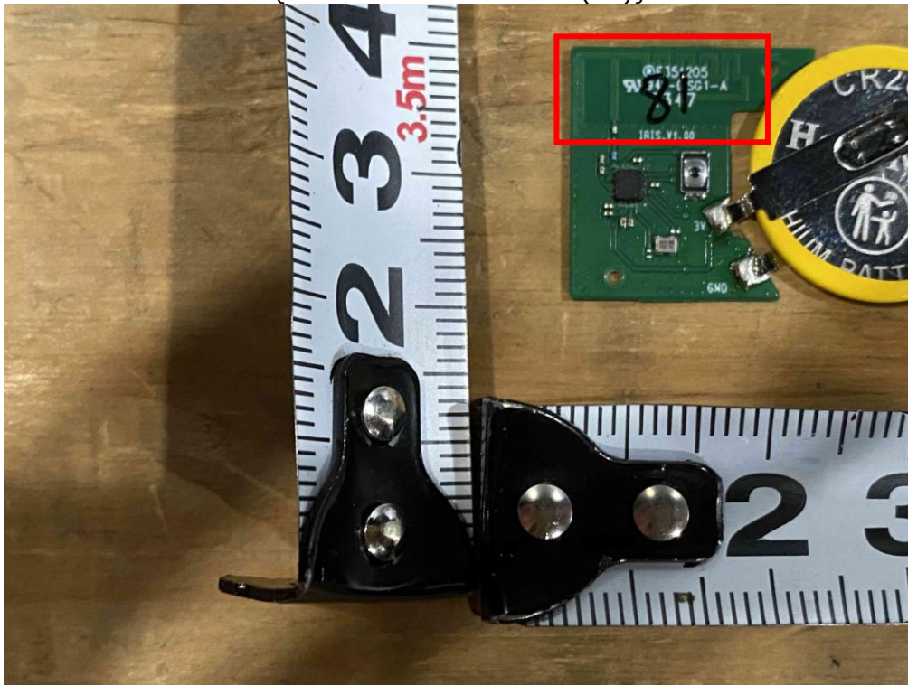
{2402-2480MHz Antenna(TX)}
