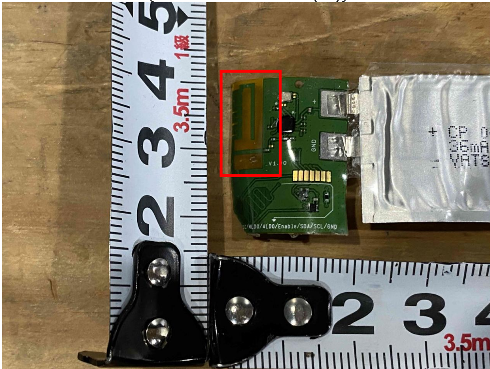
{2402-2480MHz Antenna(TX)}
