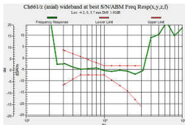
Fig 7.2 GSM1900 Ch661
