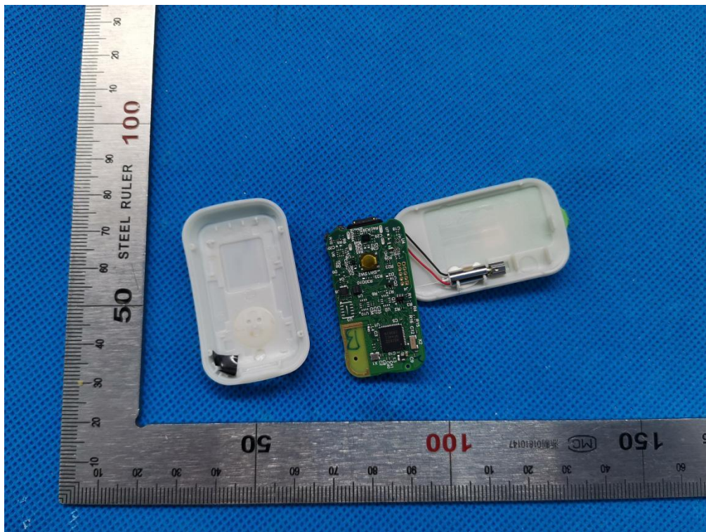
Series Model: UR-02C-02B OPEN VIEW OF EUT
