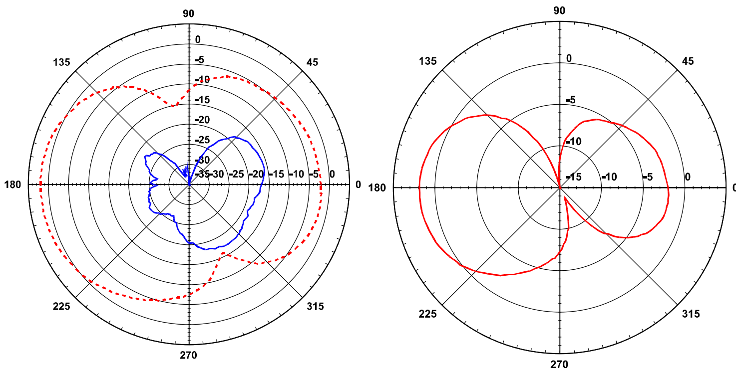
Co-cross polarization field (dBi)
