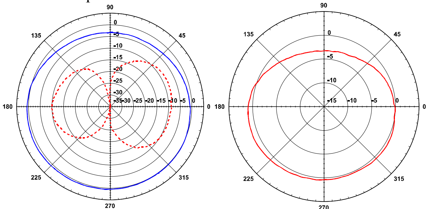
Co-cross polarization field (dBi)
