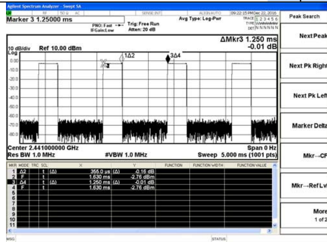
DH1-2441MHz
