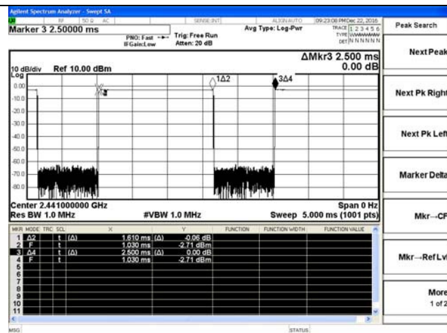
DH3-2441MHz
