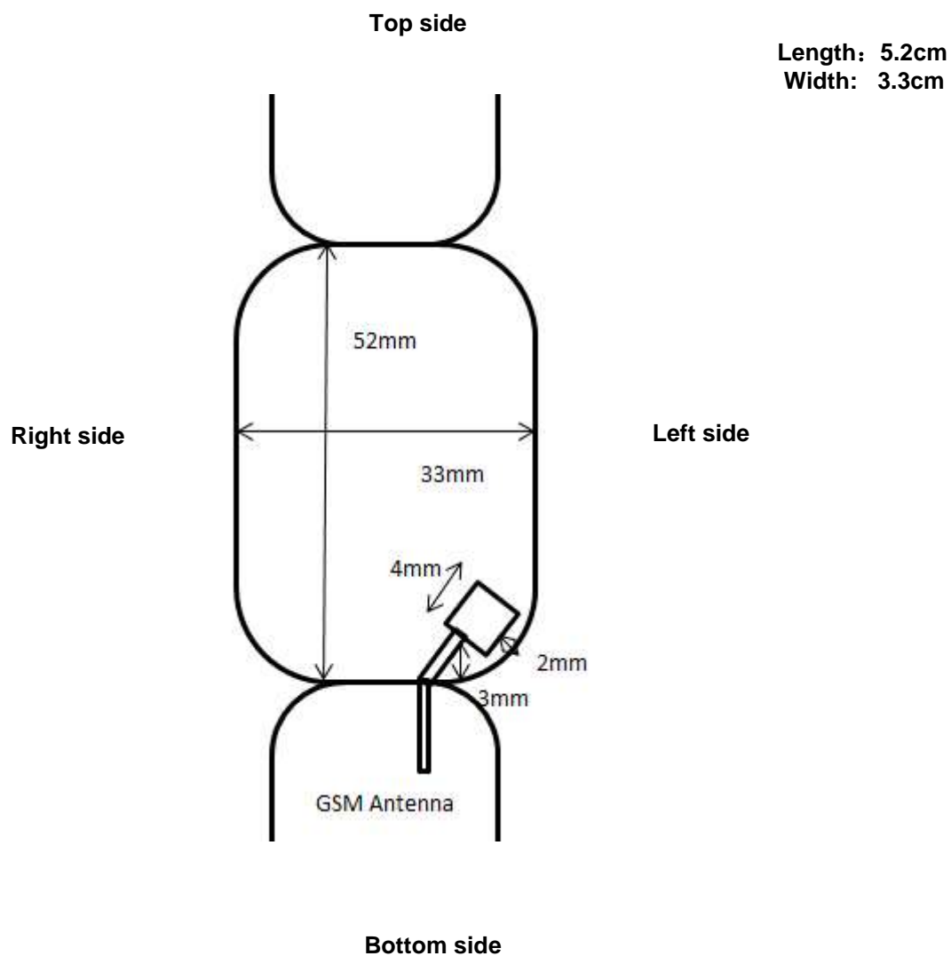
Figure1: The antenna position of the DUT
