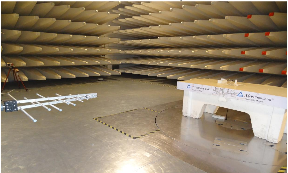
Horizontal Polarization with Adaptor 2
