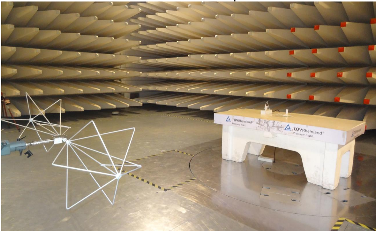
Horizontal Polarization with Adaptor 1
