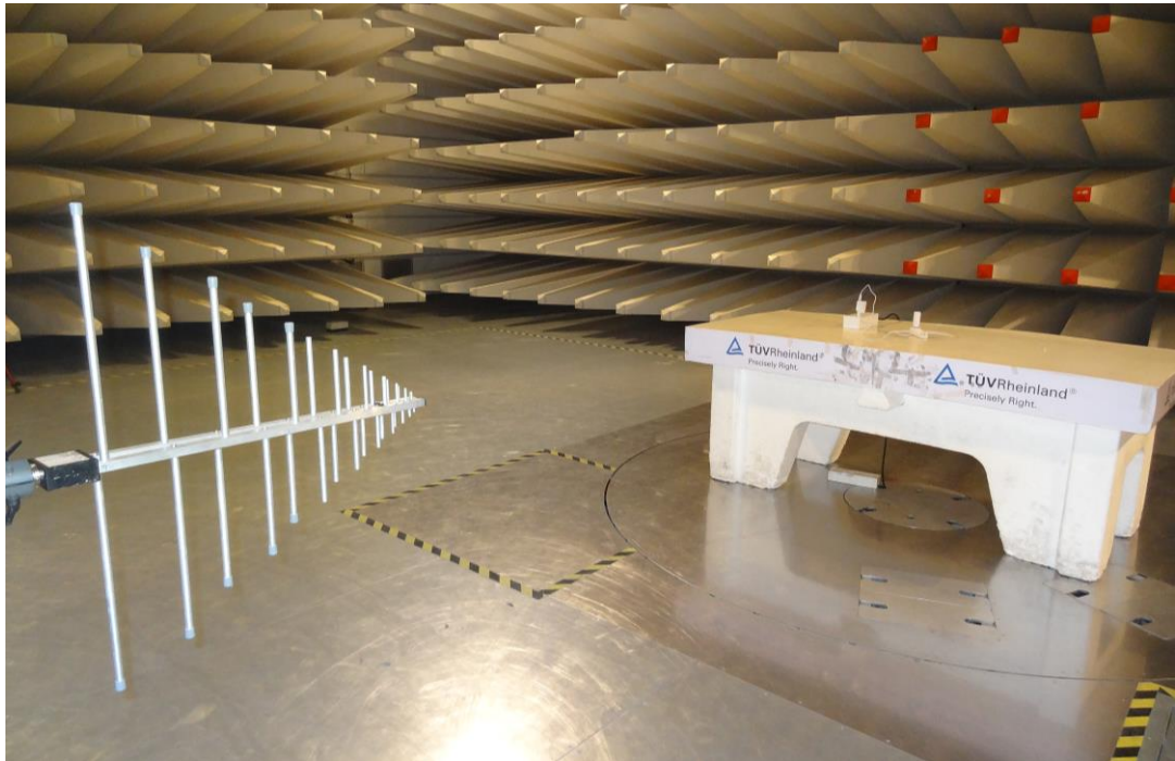
Vertical Polarization with Adaptor 1
