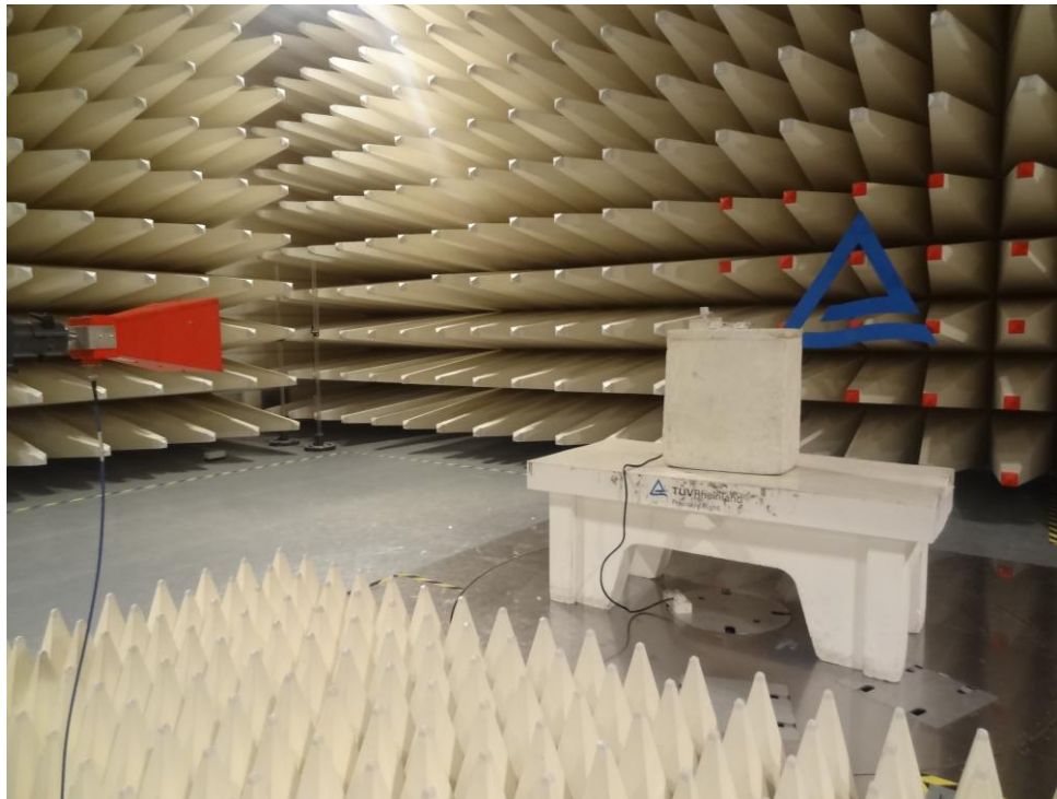
Test Setup
