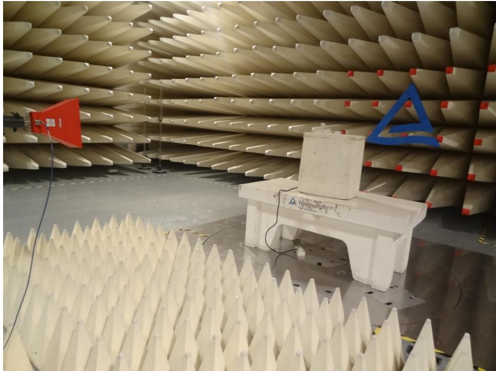
Test setup
