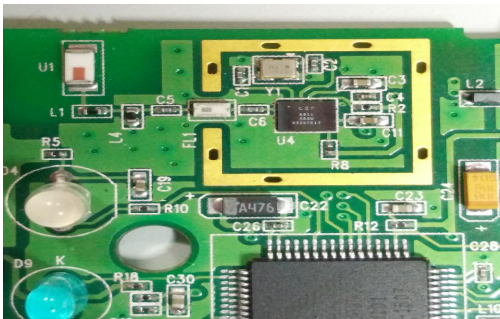
EUT RF Module with shield
