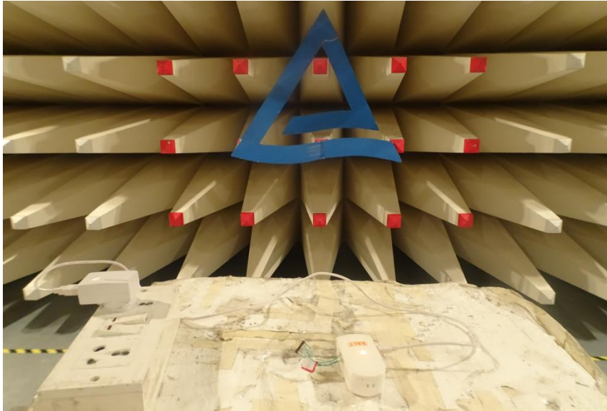
Photo 13: EUT setup
