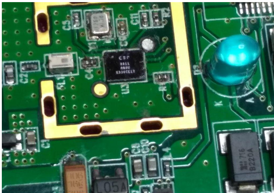
Photo 6: RF Module with shielding removed
