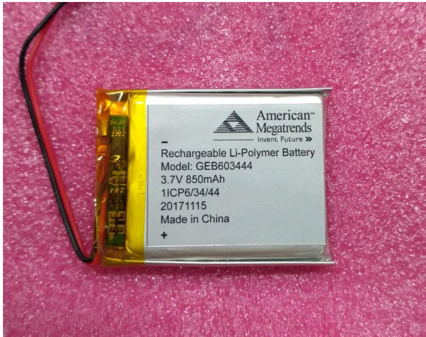
Photo 7: EUT Battery 1
