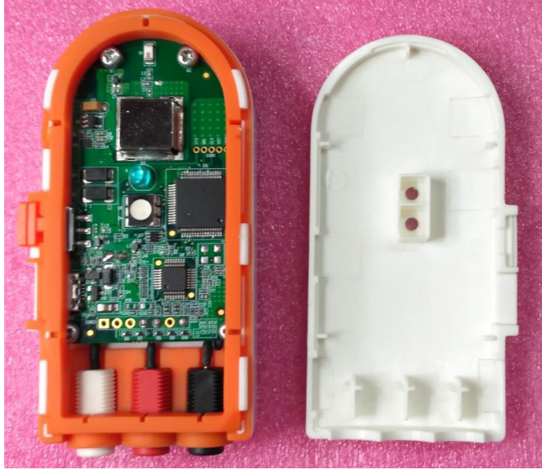
Photo 1: EUT Top Panel removed
