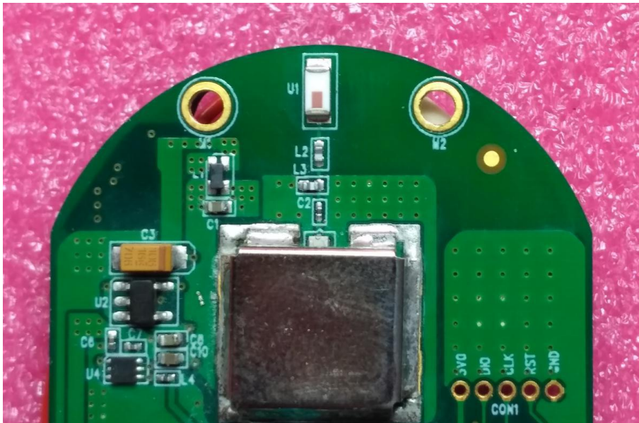
Photo 5: RF Module with shield
